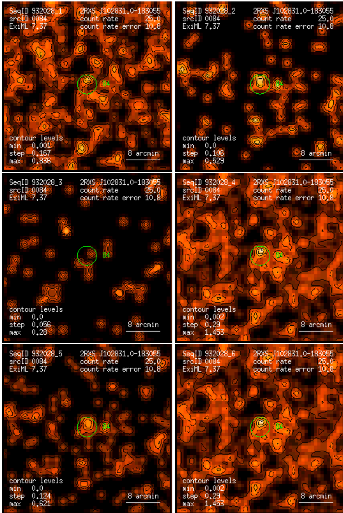
Figure 84: RASS 932028: detection 0084: band rate images, Gaussian filter: (1) PSPC channels 11 – 41, (2) 52 – 90, (3) 91 – 201, (4) 11 – 235, (5) 52 – 201, (6) 11 – 201. Broad band rates in counts/ks. Band rate contour levels in counts/ks/arcmin 2 .
