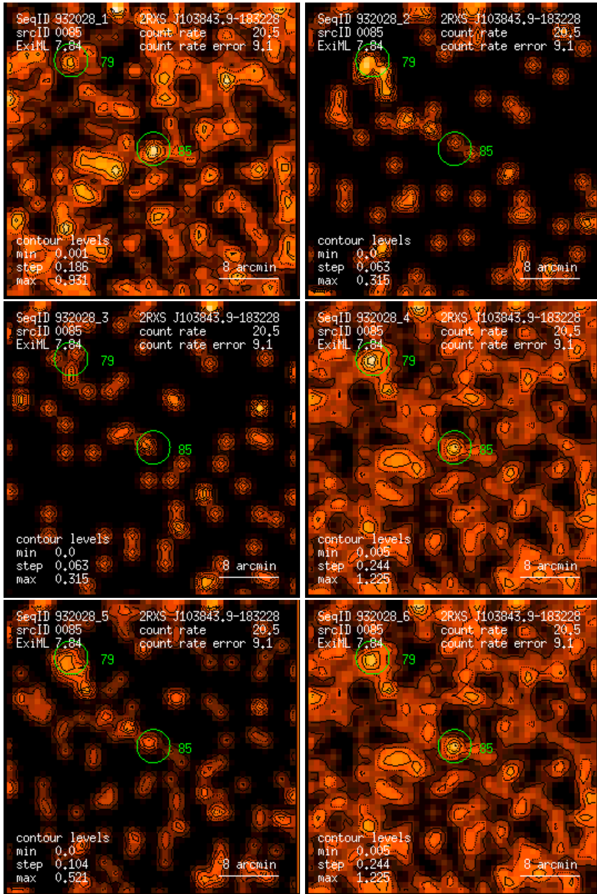
Figure 85: RASS 932028: detection 0085: band rate images, Gaussian filter: (1) PSPC channels 11 – 41, (2) 52 – 90, (3) 91 – 201, (4) 11 – 235, (5) 52 – 201, (6) 11 – 201. Broad band rates in counts/ks. Band rate contour levels in counts/ks/arcmin 2 .
