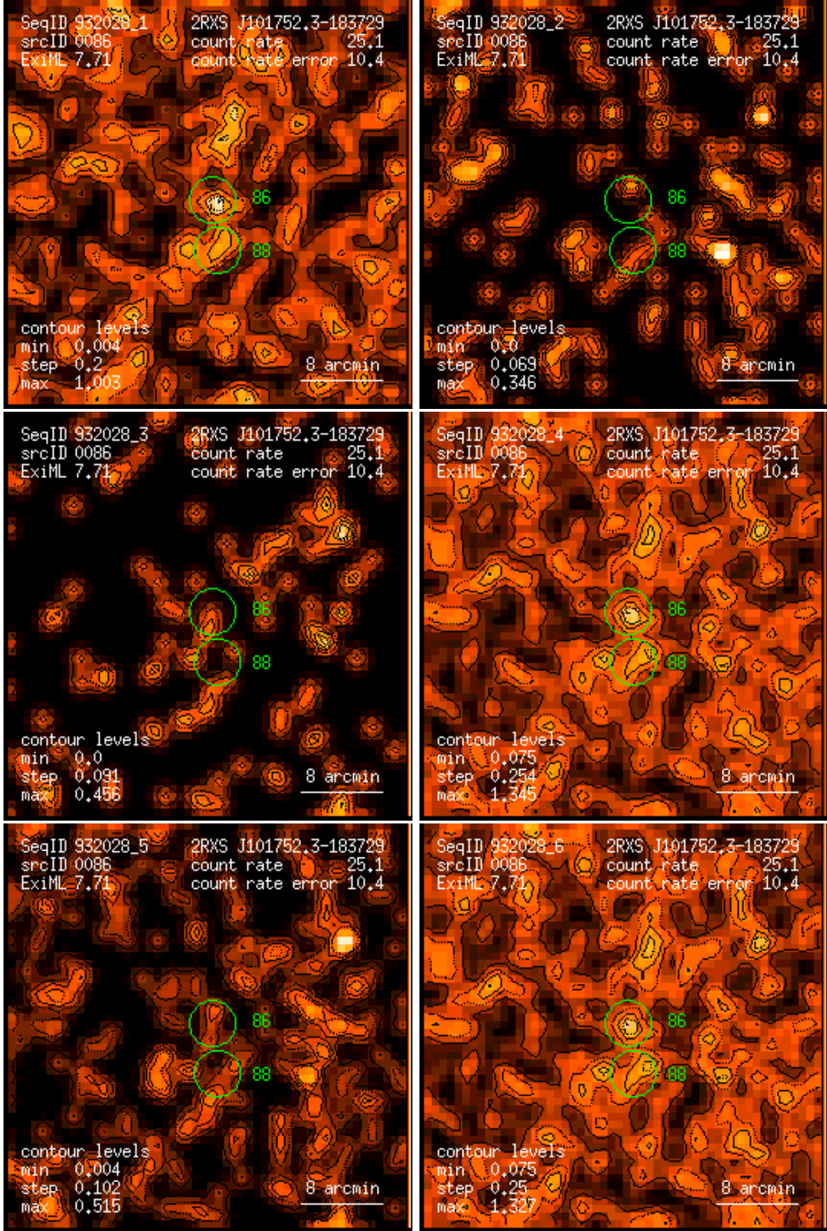
Figure 86: RASS 932028: detection 0086: band rate images, Gaussian filter: (1) PSPC channels 11 – 41, (2) 52 – 90, (3) 91 – 201, (4) 11 – 235, (5) 52 – 201, (6) 11 – 201. Broad band rates in counts/ks. Band rate contour levels in counts/ks/arcmin 2 .
