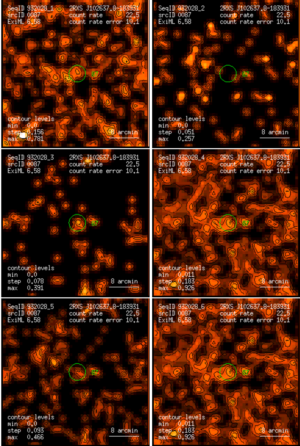
Figure 87: RASS 932028: detection 0087: band rate images, Gaussian filter: (1) PSPC channels 11 – 41, (2) 52 – 90, (3) 91 – 201, (4) 11 – 235, (5) 52 – 201, (6) 11 – 201. Broad band rates in counts/ks. Band rate contour levels in counts/ks/arcmin 2 .
