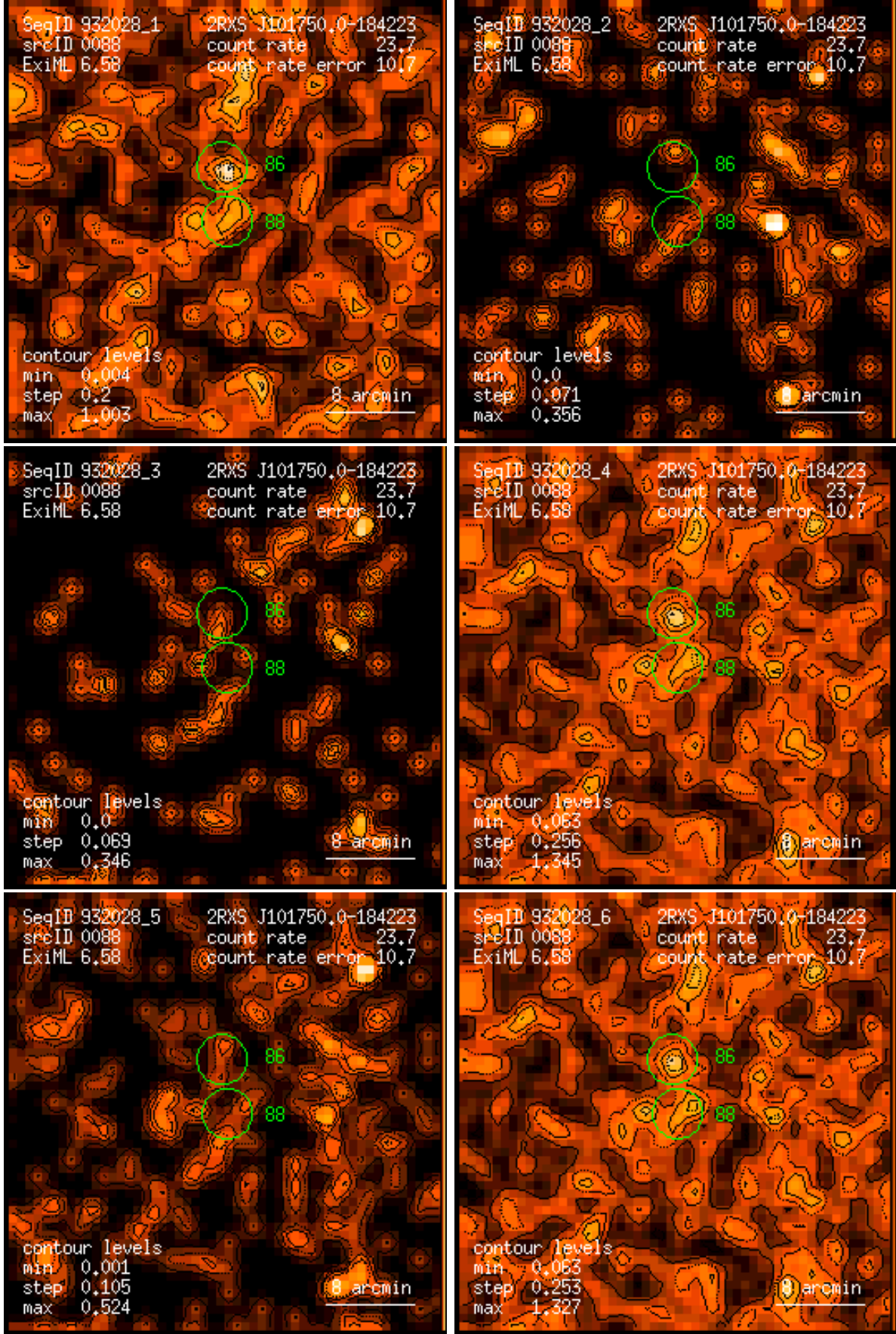
Figure 88: RASS 932028: detection 0088: band rate images, Gaussian filter: (1) PSPC channels 11 – 41, (2) 52 – 90, (3) 91 – 201, (4) 11 – 235, (5) 52 – 201, (6) 11 – 201. Broad band rates in counts/ks. Band rate contour levels in counts/ks/arcmin 2 .
