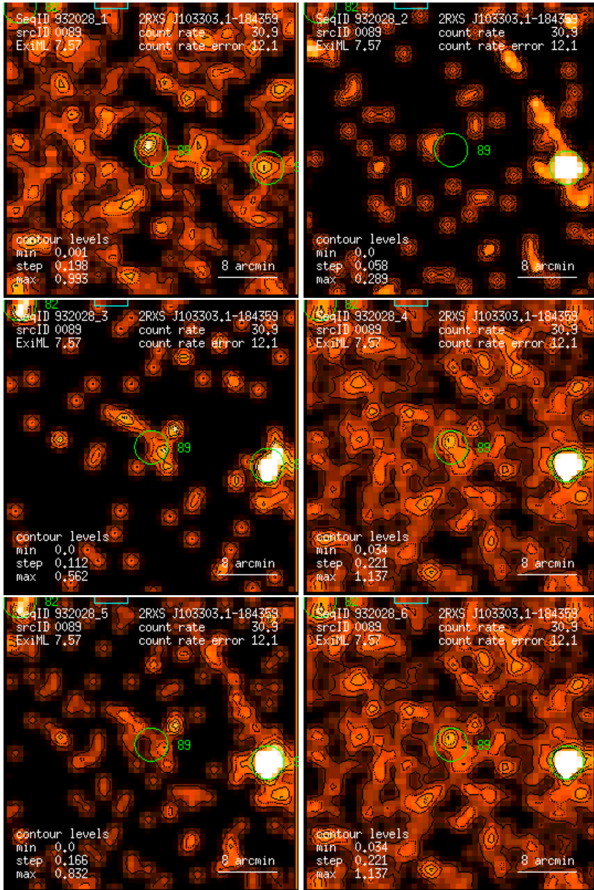
Figure 89: RASS 932028: detection 0089: band rate images, Gaussian filter: (1) PSPC channels 11 – 41, (2) 52 – 90, (3) 91 – 201, (4) 11 – 235, (5) 52 – 201, (6) 11 – 201. Broad band rates in counts/ks. Band rate contour levels in counts/ks/arcmin 2 .
