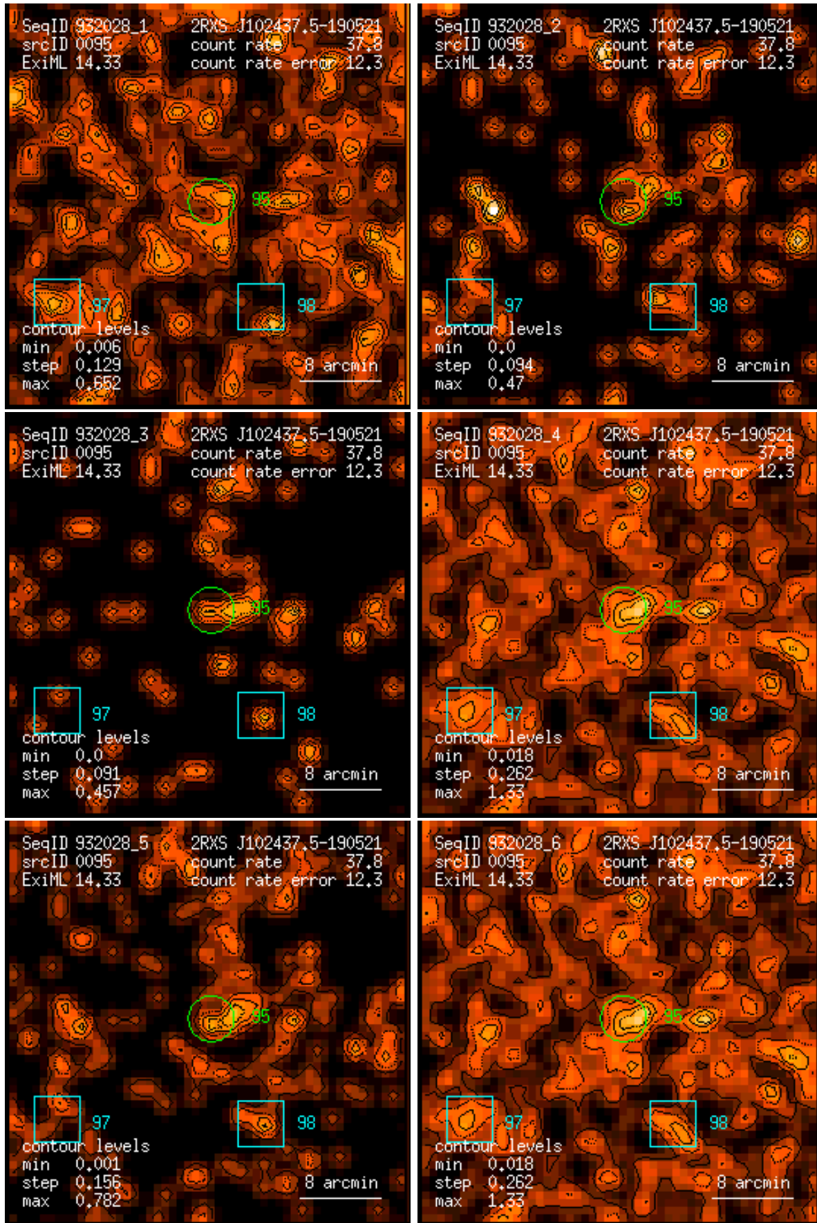
Figure 95: RASS 932028: detection 0095: band rate images, Gaussian filter: (1) PSPC channels 11 – 41, (2) 52 – 90, (3) 91 – 201, (4) 11 – 235, (5) 52 – 201, (6) 11 – 201. Broad band rates in counts/ks. Band rate contour levels in counts/ks/arcmin 2 .
