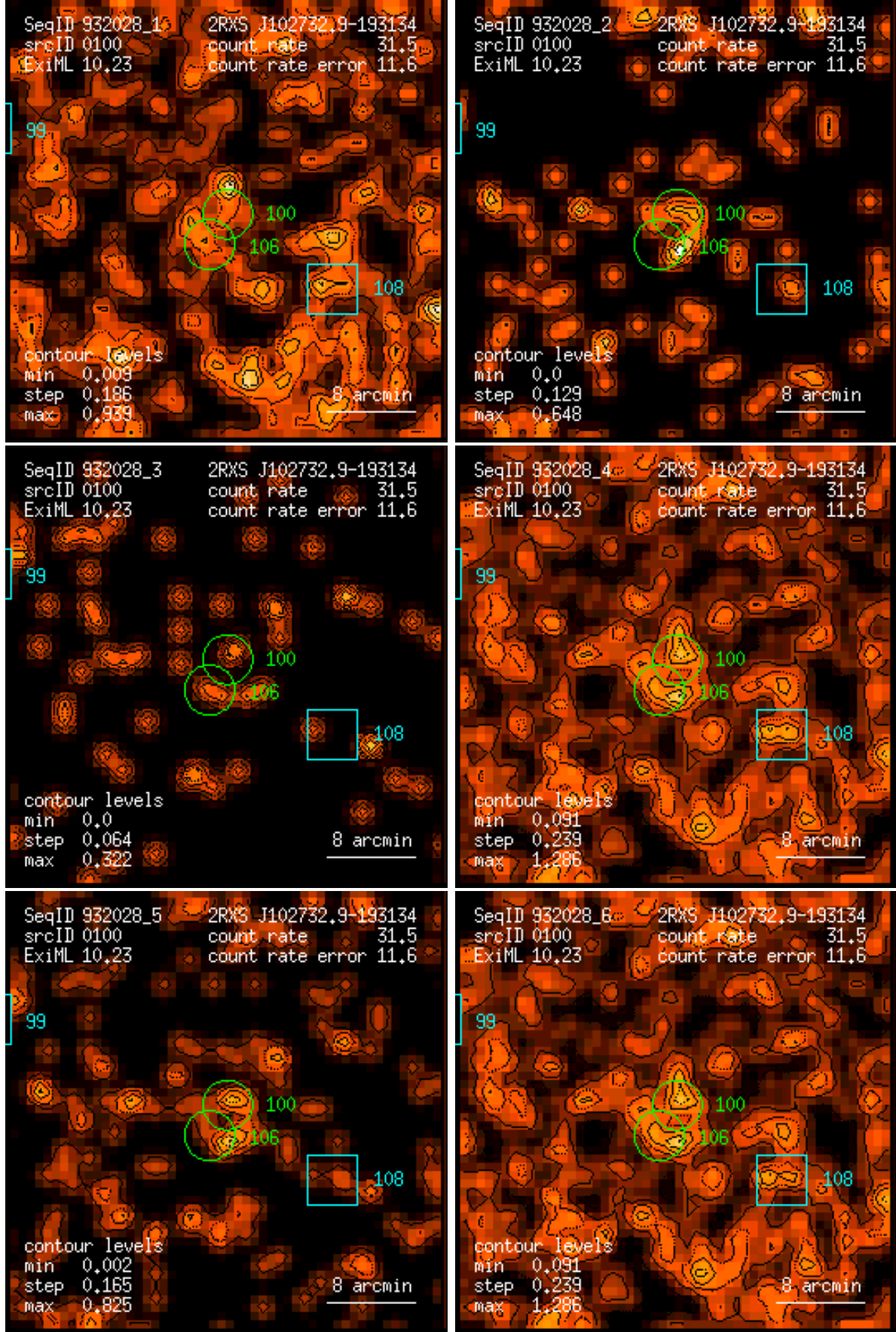
Figure 100: RASS 932028: detection 0100: band rate images, Gaussian filter: (1) PSPC channels 11 – 41, (2) 52 – 90, (3) 91 – 201, (4) 11 – 235, (5) 52 – 201, (6) 11 – 201. Broad band rates in counts/ks. Band rate contour levels in counts/ks/arcmin 2 .
