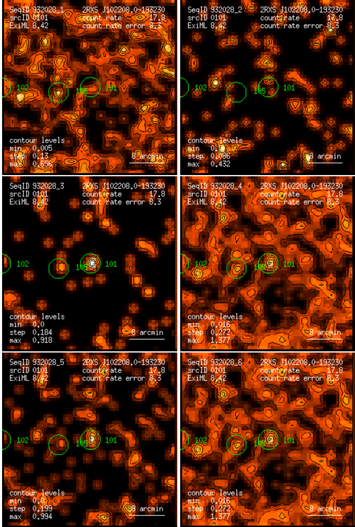
Figure 101: RASS 932028: detection 0101: band rate images, Gaussian filter: (1) PSPC channels 11 – 41, (2) 52 – 90, (3) 91 – 201, (4) 11 – 235, (5) 52 – 201, (6) 11 – 201. Broad band rates in counts/ks. Band rate contour levels in counts/ks/arcmin 2 .
