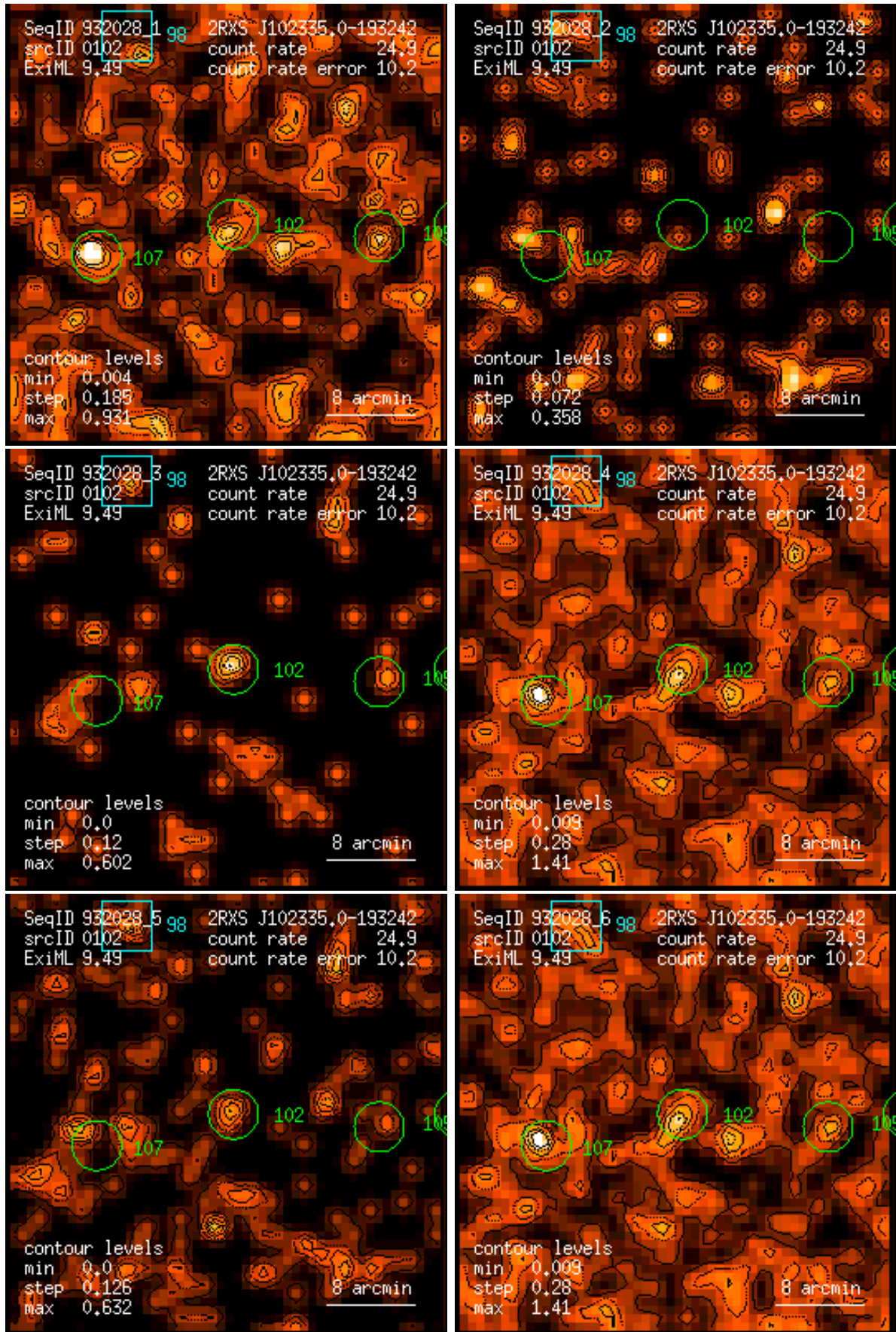
Figure 102: RASS 932028: detection 0102: band rate images, Gaussian filter: (1) PSPC channels 11 – 41, (2) 52 – 90, (3) 91 – 201, (4) 11 – 235, (5) 52 – 201, (6) 11 – 201. Broad band rates in counts/ks. Band rate contour levels in counts/ks/arcmin 2 .
