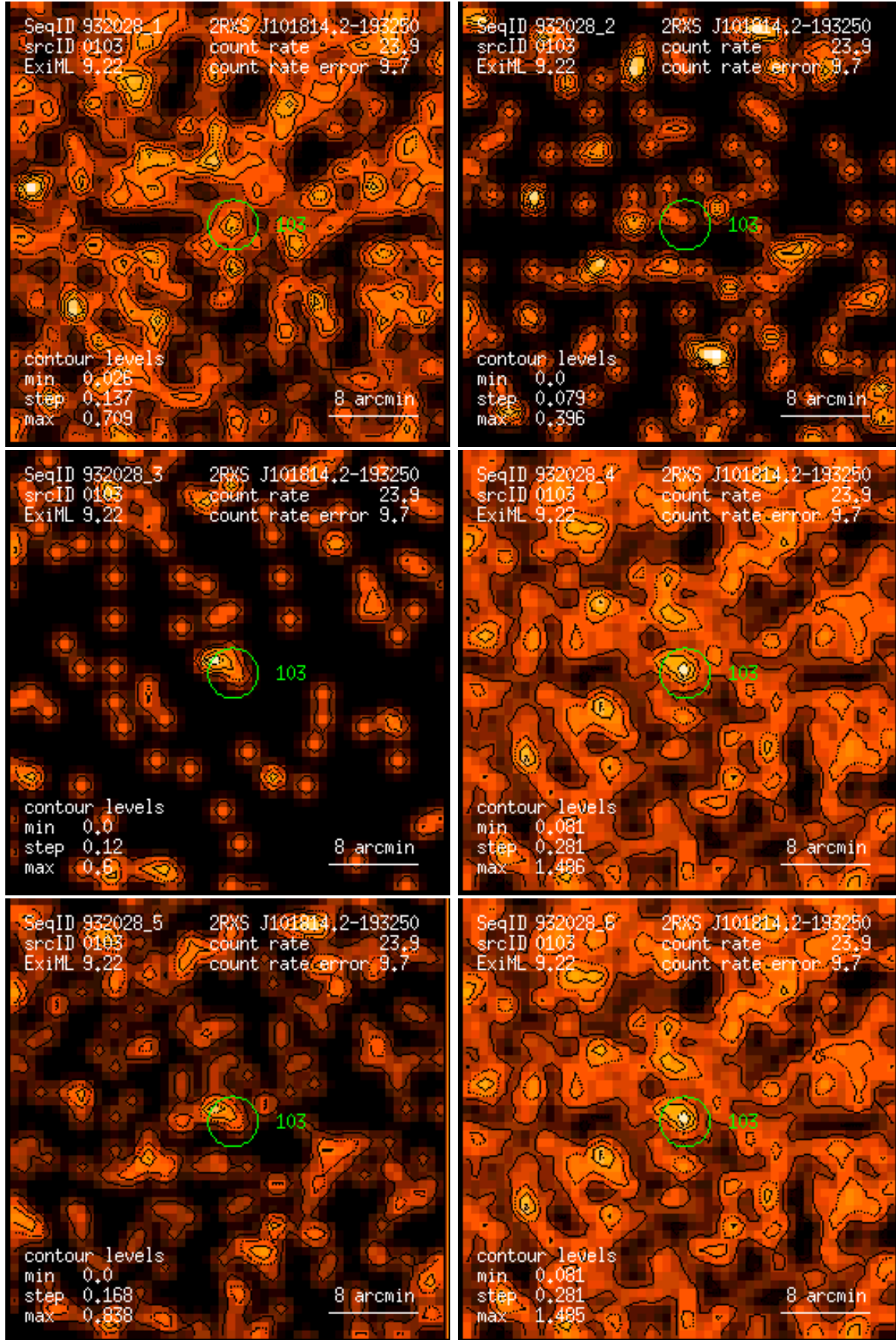
Figure 103: RASS 932028: detection 0103: band rate images, Gaussian filter: (1) PSPC channels 11 – 41, (2) 52 – 90, (3) 91 – 201, (4) 11 – 235, (5) 52 – 201, (6) 11 – 201. Broad band rates in counts/ks. Band rate contour levels in counts/ks/arcmin 2 .
