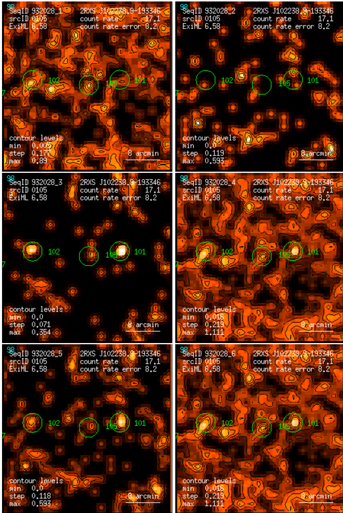
Figure 105: RASS 932028: detection 0105: band rate images, Gaussian filter: (1) PSPC channels 11 – 41, (2) 52 – 90, (3) 91 – 201, (4) 11 – 235, (5) 52 – 201, (6) 11 – 201. Broad band rates in counts/ks. Band rate contour levels in counts/ks/arcmin 2 .
