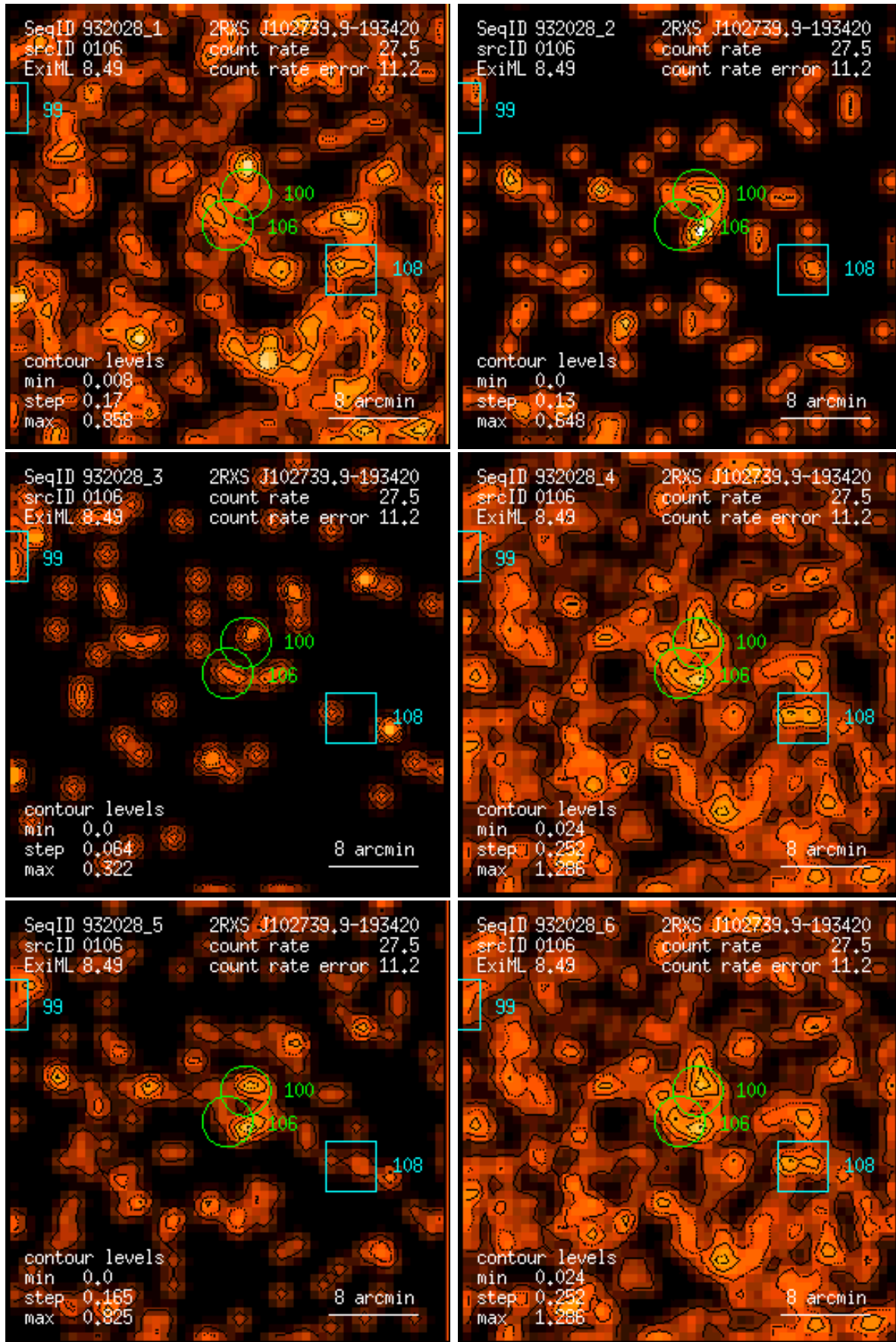
Figure 106: RASS 932028: detection 0106: band rate images, Gaussian filter: (1) PSPC channels 11 – 41, (2) 52 – 90, (3) 91 – 201, (4) 11 – 235, (5) 52 – 201, (6) 11 – 201. Broad band rates in counts/ks. Band rate contour levels in counts/ks/arcmin 2 .
