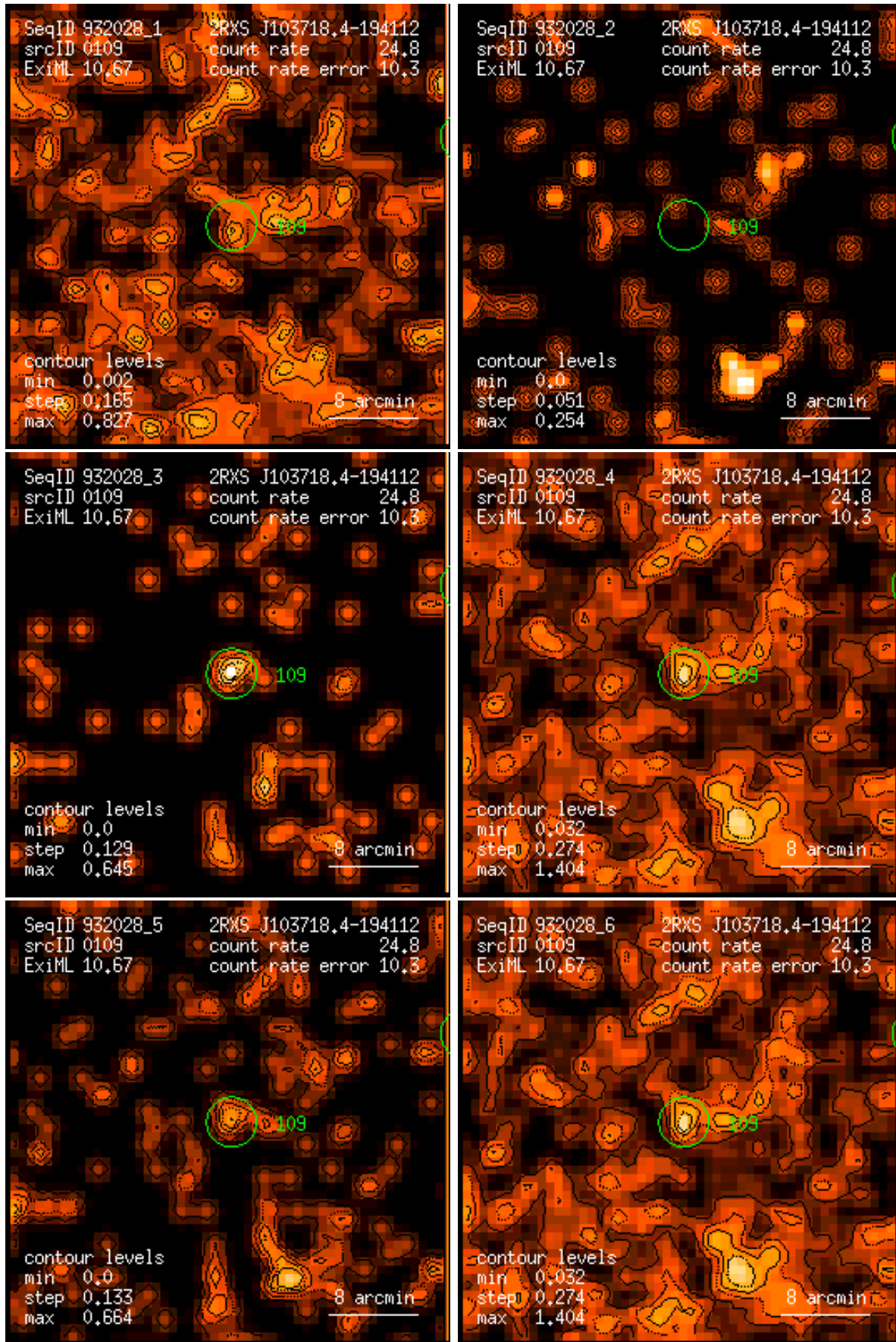
Figure 109: RASS 932028: detection 0109: band rate images, Gaussian filter: (1) PSPC channels 11 – 41, (2) 52 – 90, (3) 91 – 201, (4) 11 – 235, (5) 52 – 201, (6) 11 – 201. Broad band rates in counts/ks. Band rate contour levels in counts/ks/arcmin 2 .
