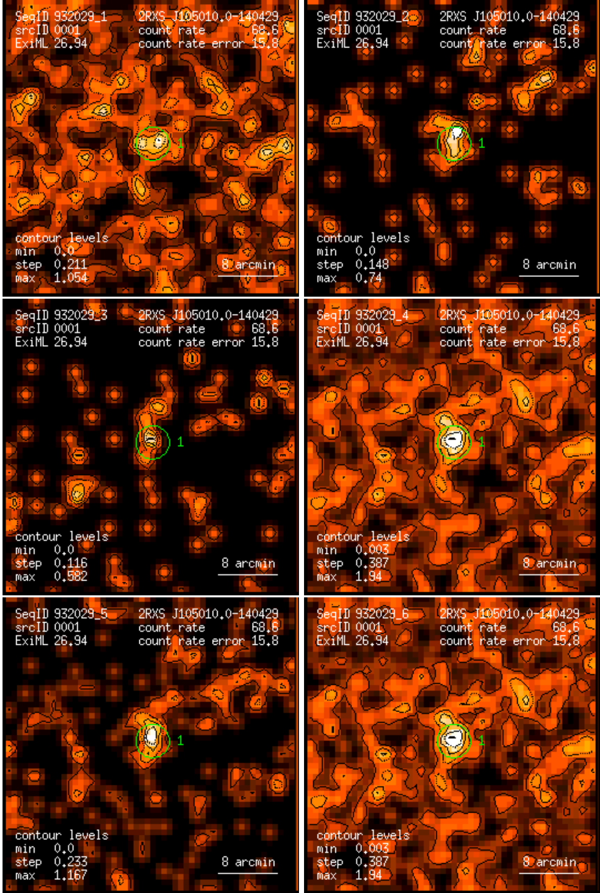
Figure 1: RASS 932029: detection 0001: band rate images, Gaussian filter: (1) PSPC channels 11 – 41, (2) 52 – 90, (3) 91 – 201, (4) 11 – 235, (5) 52 – 201, (6) 11 – 201. Broad band rates in counts/ks. Band rate contour levels in counts/ks/arcmin 2 .
