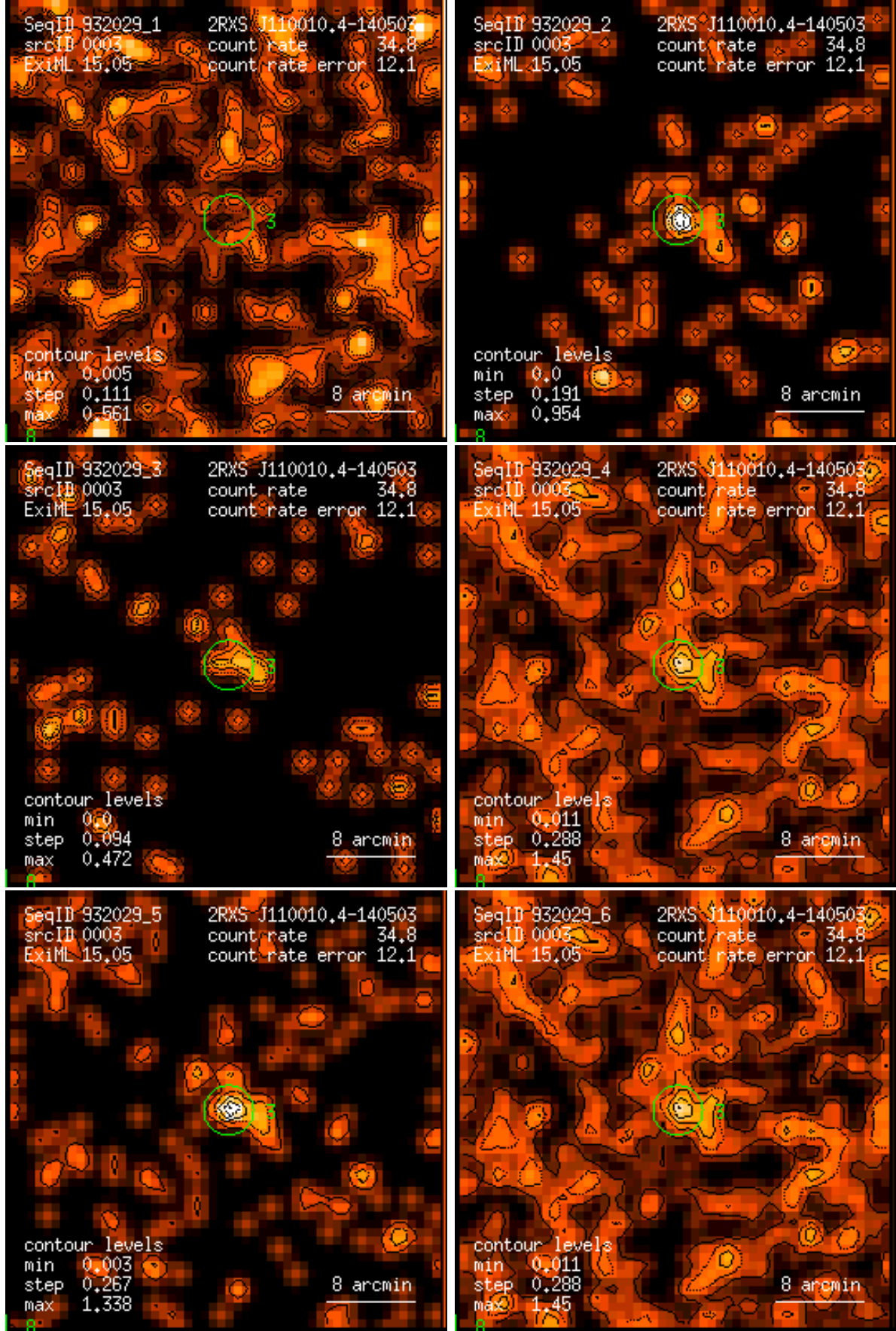
Figure 3: RASS 932029: detection 0003: band rate images, Gaussian filter: (1) PSPC channels 11 – 41, (2) 52 – 90, (3) 91 – 201, (4) 11 – 235, (5) 52 – 201, (6) 11 – 201. Broad band rates in counts/ks. Band rate contour levels in counts/ks/arcmin 2 .
