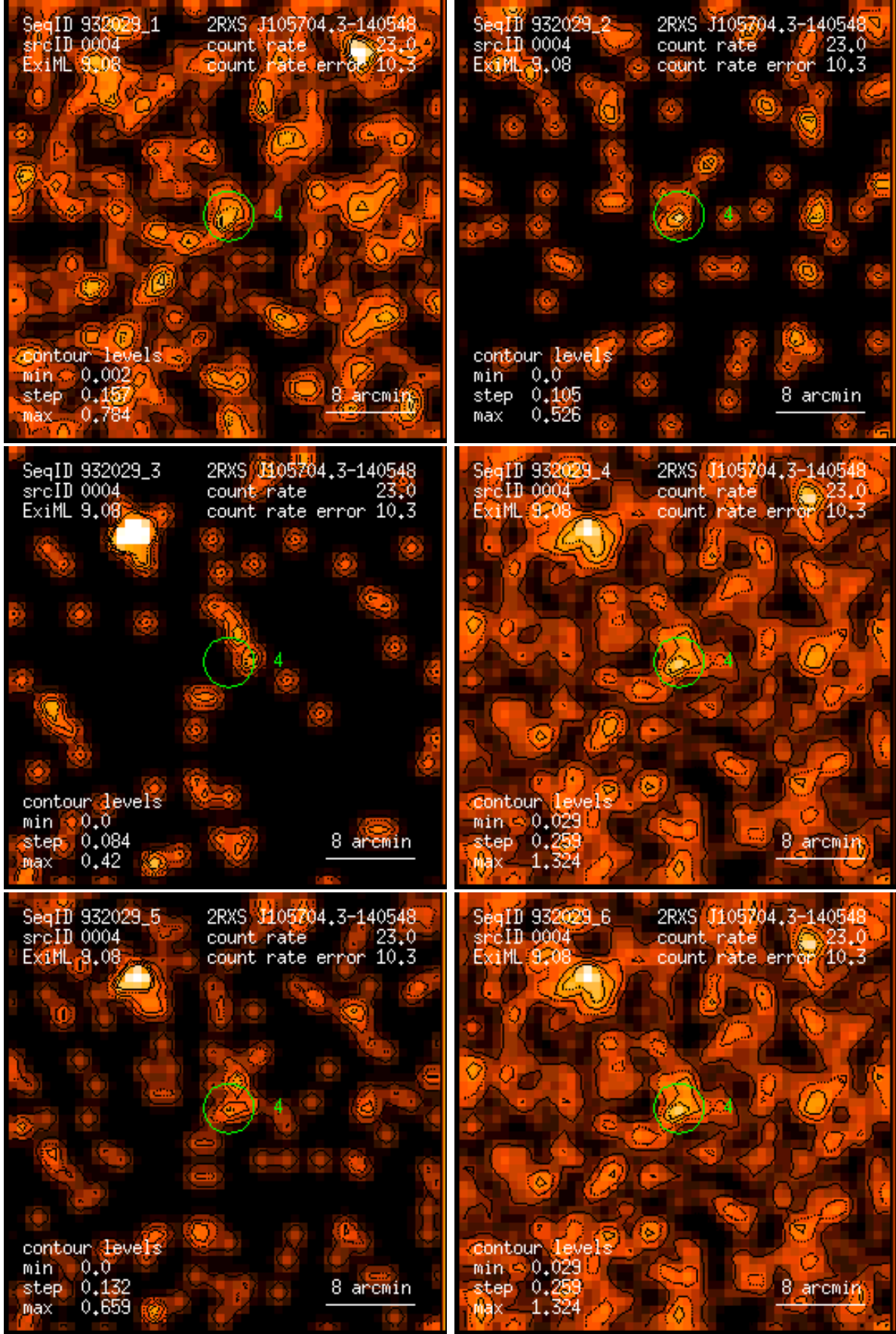
Figure 4: RASS 932029: detection 0004: band rate images, Gaussian filter: (1) PSPC channels 11 – 41, (2) 52 – 90, (3) 91 – 201, (4) 11 – 235, (5) 52 – 201, (6) 11 – 201. Broad band rates in counts/ks. Band rate contour levels in counts/ks/arcmin 2 .
