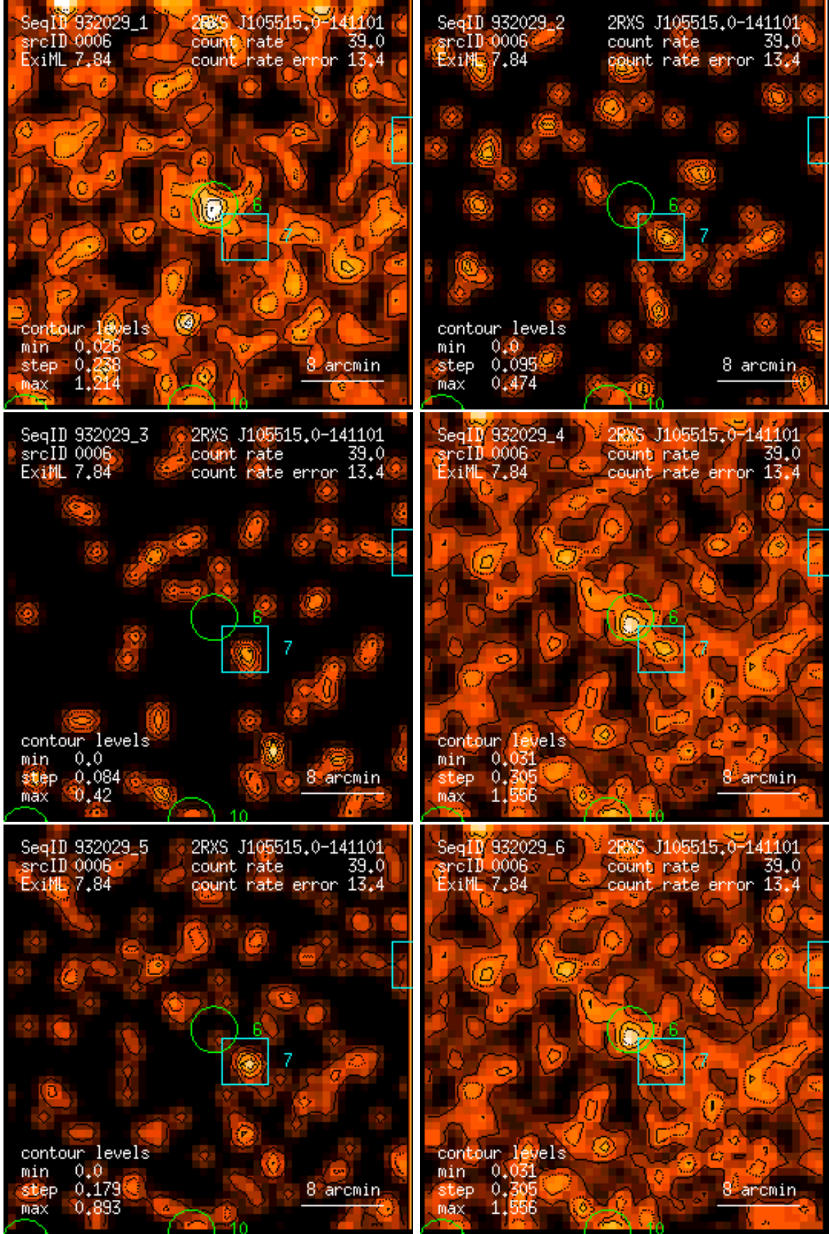
Figure 6: RASS 932029: detection 0006: band rate images, Gaussian filter: (1) PSPC channels 11 – 41, (2) 52 – 90, (3) 91 – 201, (4) 11 – 235, (5) 52 – 201, (6) 11 – 201. Broad band rates in counts/ks. Band rate contour levels in counts/ks/arcmin 2 .
