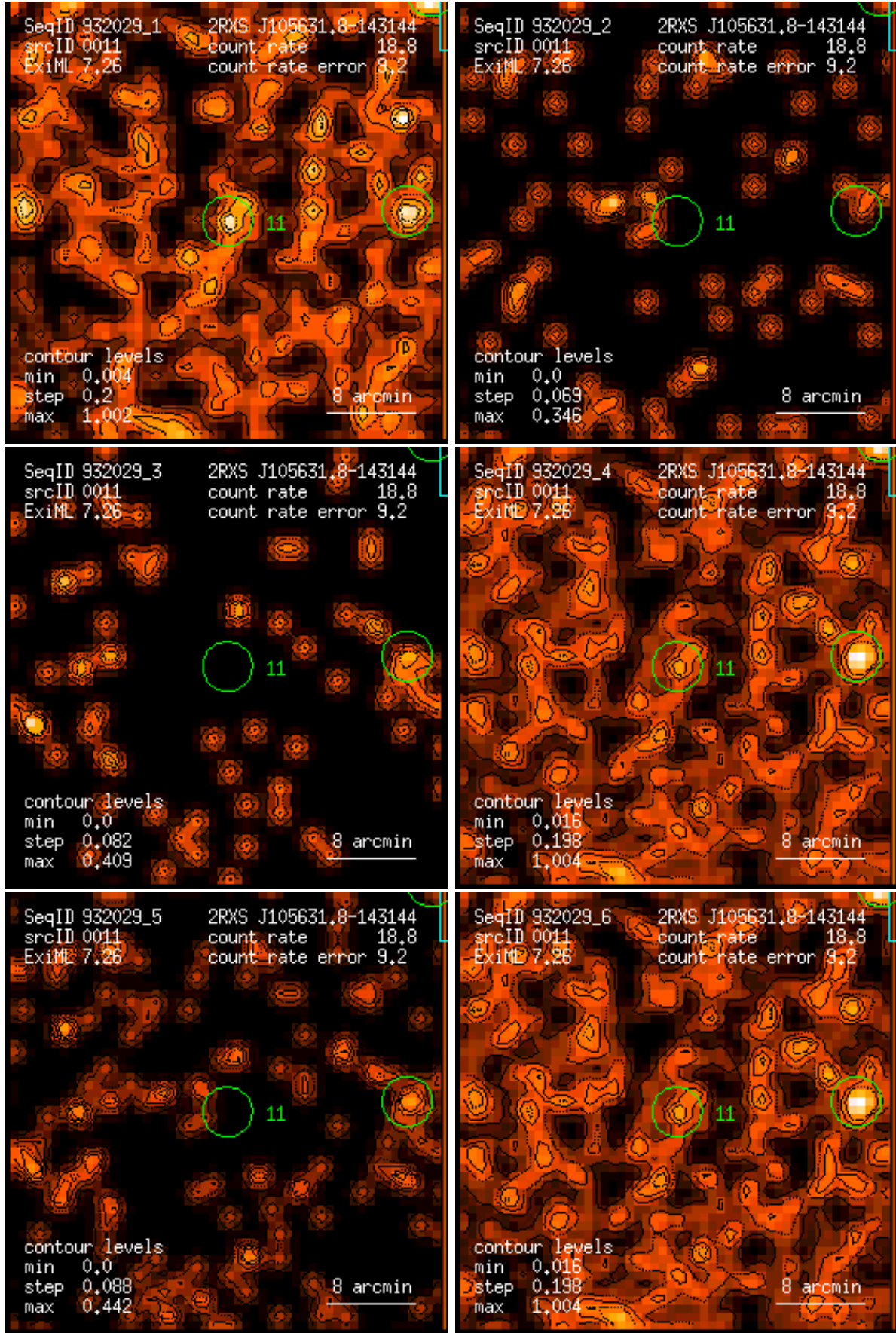
Figure 11: RASS 932029: detection 0011: band rate images, Gaussian filter: (1) PSPC channels 11 – 41, (2) 52 – 90, (3) 91 – 201, (4) 11 – 235, (5) 52 – 201, (6) 11 – 201. Broad band rates in counts/ks. Band rate contour levels in counts/ks/arcmin 2 .
