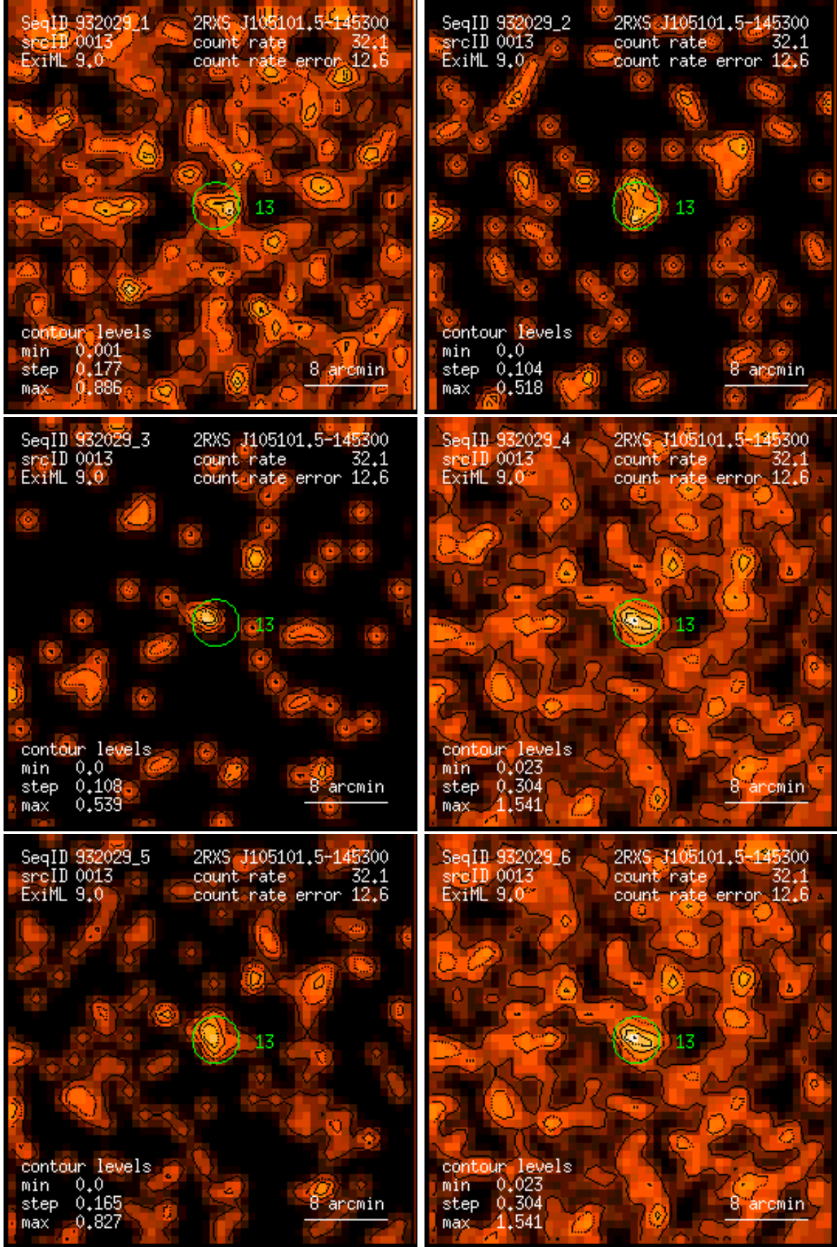
Figure 13: RASS 932029: detection 0013: band rate images, Gaussian filter: (1) PSPC channels 11 – 41, (2) 52 – 90, (3) 91 – 201, (4) 11 – 235, (5) 52 – 201, (6) 11 – 201. Broad band rates in counts/ks. Band rate contour levels in counts/ks/arcmin 2 .
