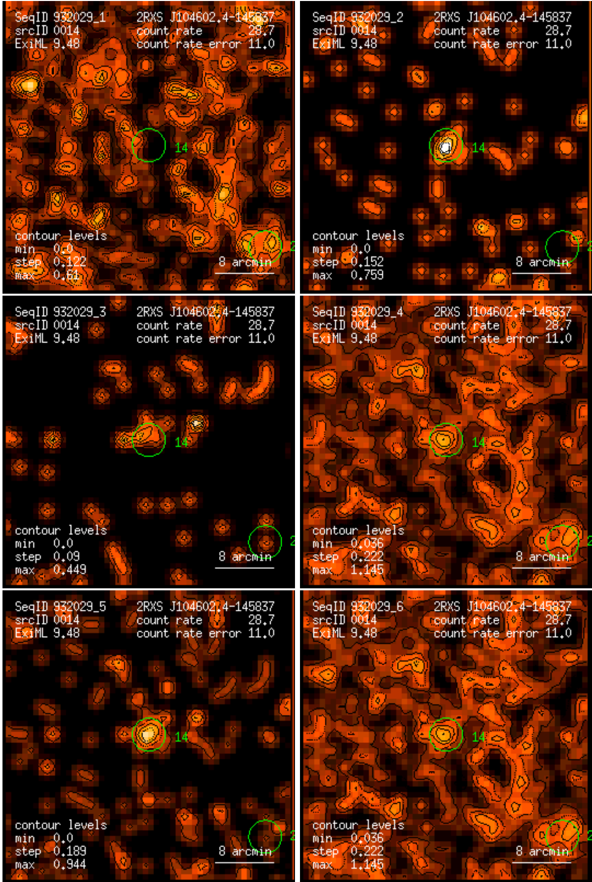
Figure 14: RASS 932029: detection 0014: band rate images, Gaussian filter: (1) PSPC channels 11 – 41, (2) 52 – 90, (3) 91 – 201, (4) 11 – 235, (5) 52 – 201, (6) 11 – 201. Broad band rates in counts/ks. Band rate contour levels in counts/ks/arcmin 2 .
