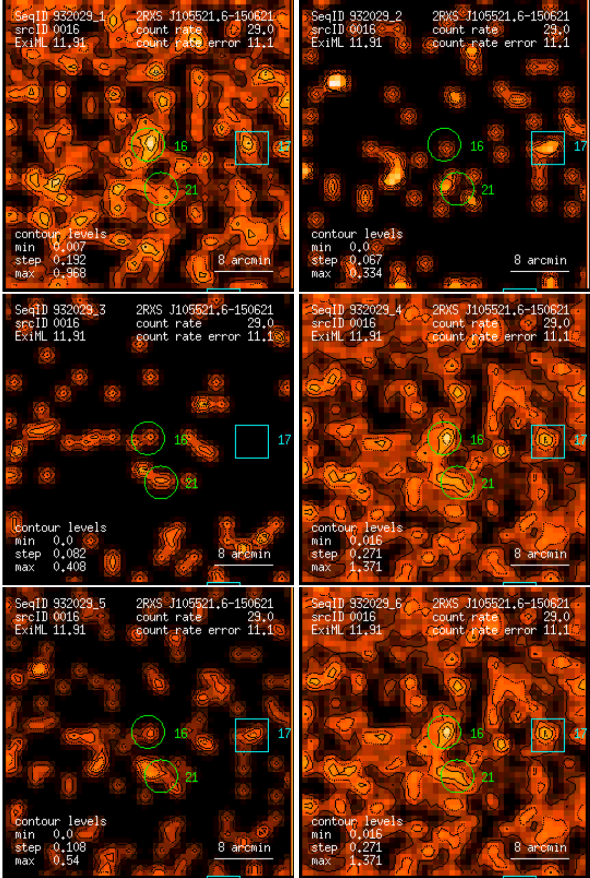
Figure 16: RASS 932029: detection 0016: band rate images, Gaussian filter: (1) PSPC channels 11 – 41, (2) 52 – 90, (3) 91 – 201, (4) 11 – 235, (5) 52 – 201, (6) 11 – 201. Broad band rates in counts/ks. Band rate contour levels in counts/ks/arcmin 2 .
