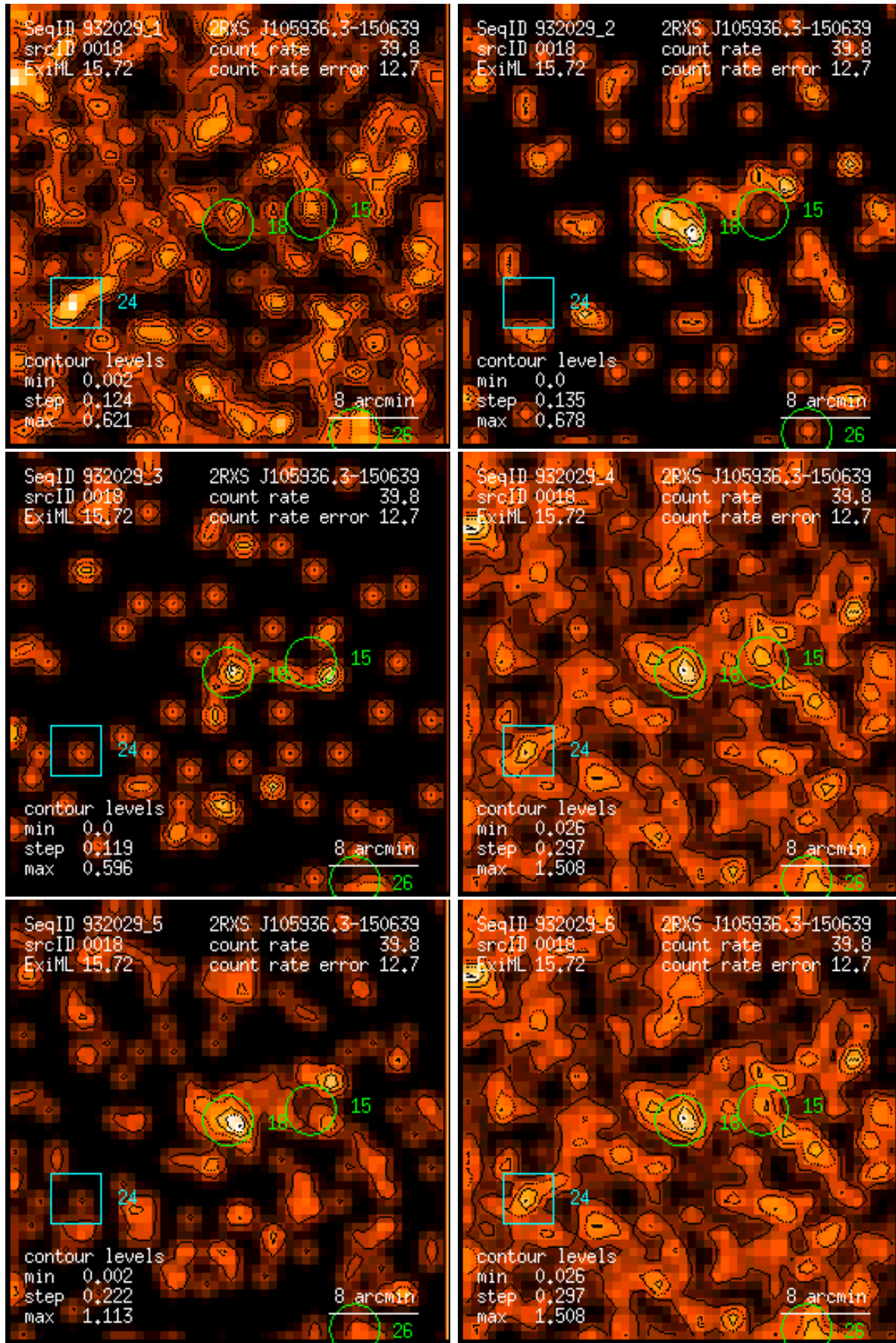
Figure 18: RASS 932029: detection 0018: band rate images, Gaussian filter: (1) PSPC channels 11 – 41, (2) 52 – 90, (3) 91 – 201, (4) 11 – 235, (5) 52 – 201, (6) 11 – 201. Broad band rates in counts/ks. Band rate contour levels in counts/ks/arcmin 2 .
