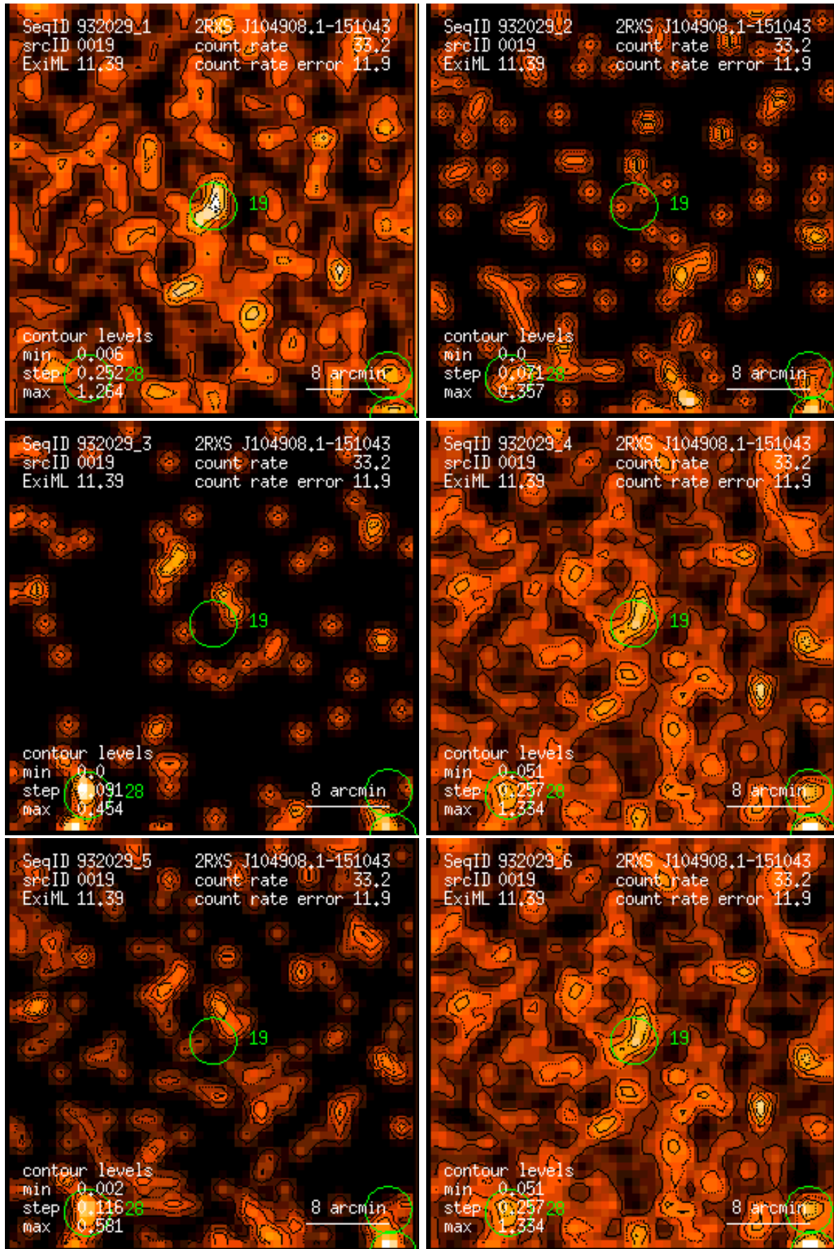
Figure 19: RASS 932029: detection 0019: band rate images, Gaussian filter: (1) PSPC channels 11 – 41, (2) 52 – 90, (3) 91 – 201, (4) 11 – 235, (5) 52 – 201, (6) 11 – 201. Broad band rates in counts/ks. Band rate contour levels in counts/ks/arcmin 2 .
