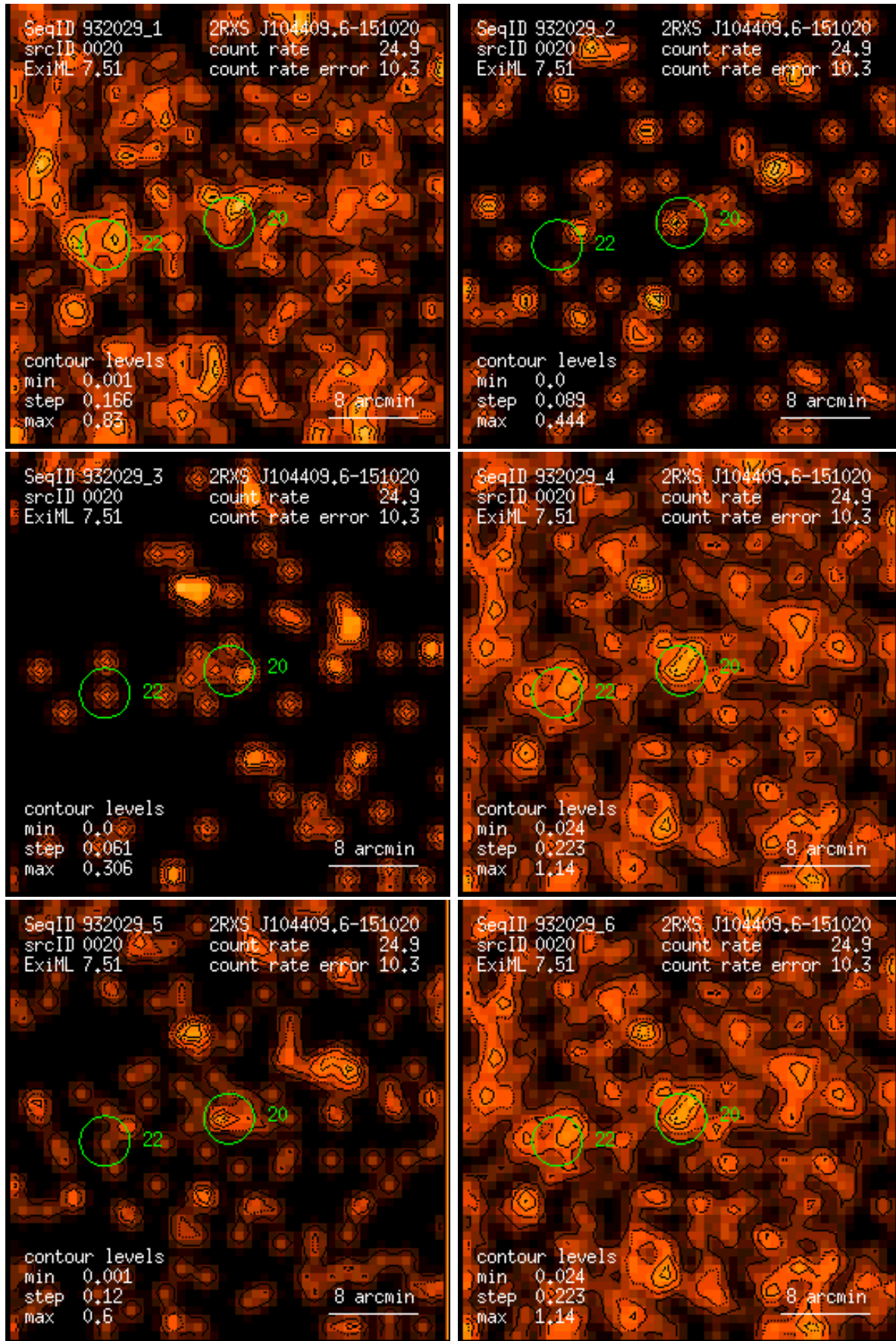
Figure 20: RASS 932029: detection 0020: band rate images, Gaussian filter: (1) PSPC channels 11 – 41, (2) 52 – 90, (3) 91 – 201, (4) 11 – 235, (5) 52 – 201, (6) 11 – 201. Broad band rates in counts/ks. Band rate contour levels in counts/ks/arcmin 2 .
