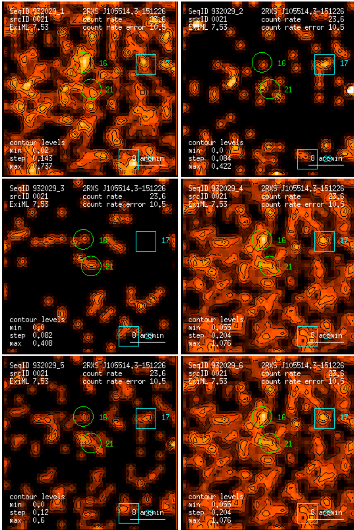
Figure 21: RASS 932029: detection 0021: band rate images, Gaussian filter: (1) PSPC channels 11 – 41, (2) 52 – 90, (3) 91 – 201, (4) 11 – 235, (5) 52 – 201, (6) 11 – 201. Broad band rates in counts/ks. Band rate contour levels in counts/ks/arcmin 2 .
