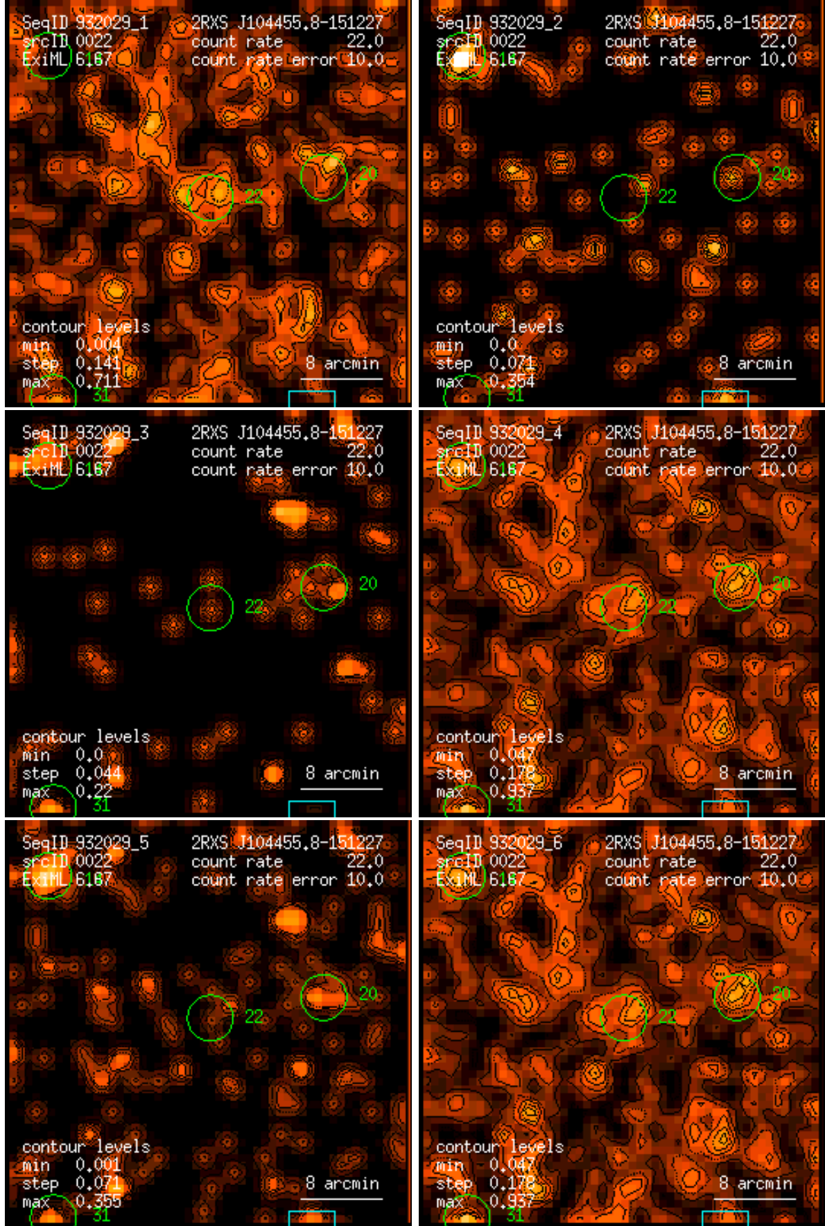
Figure 22: RASS 932029: detection 0022: band rate images, Gaussian filter: (1) PSPC channels 11 – 41, (2) 52 – 90, (3) 91 – 201, (4) 11 – 235, (5) 52 – 201, (6) 11 – 201. Broad band rates in counts/ks. Band rate contour levels in counts/ks/arcmin 2 .
