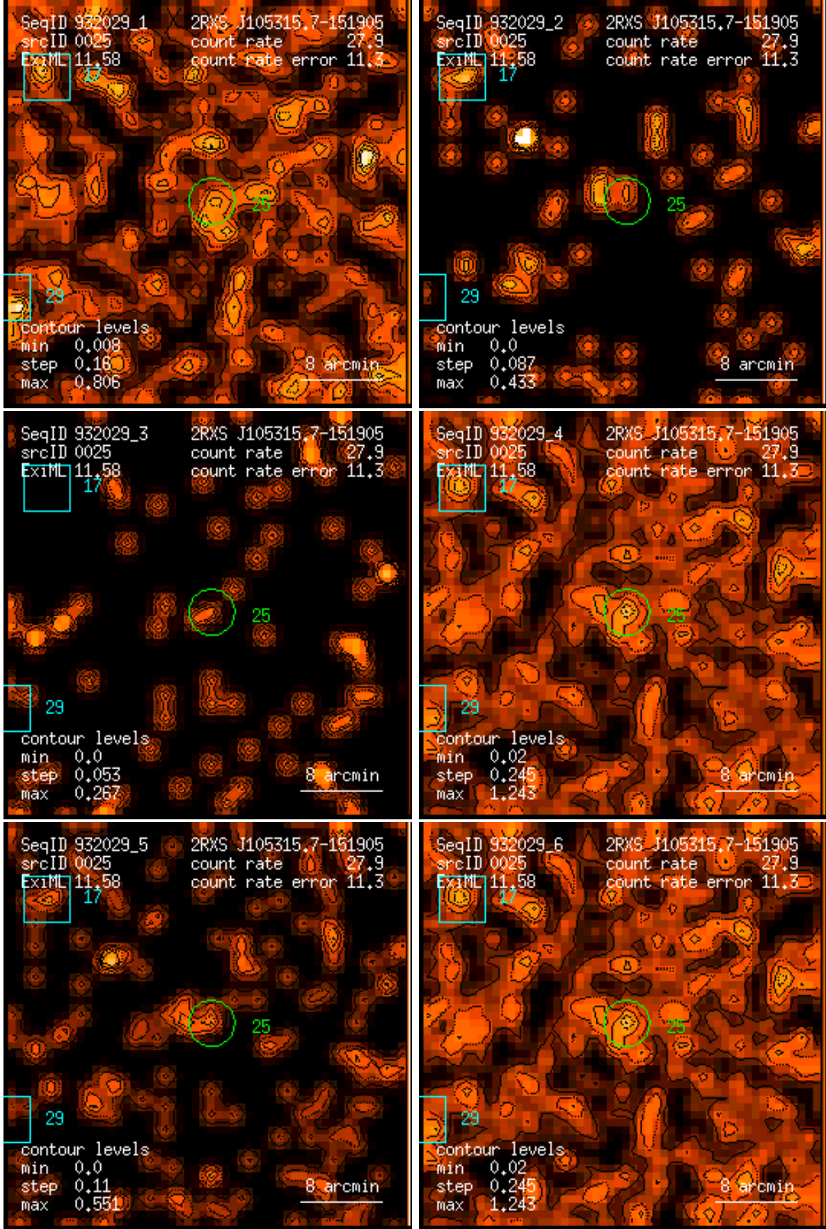
Figure 25: RASS 932029: detection 0025: band rate images, Gaussian filter: (1) PSPC channels 11 – 41, (2) 52 – 90, (3) 91 – 201, (4) 11 – 235, (5) 52 – 201, (6) 11 – 201. Broad band rates in counts/ks. Band rate contour levels in counts/ks/arcmin 2 .
