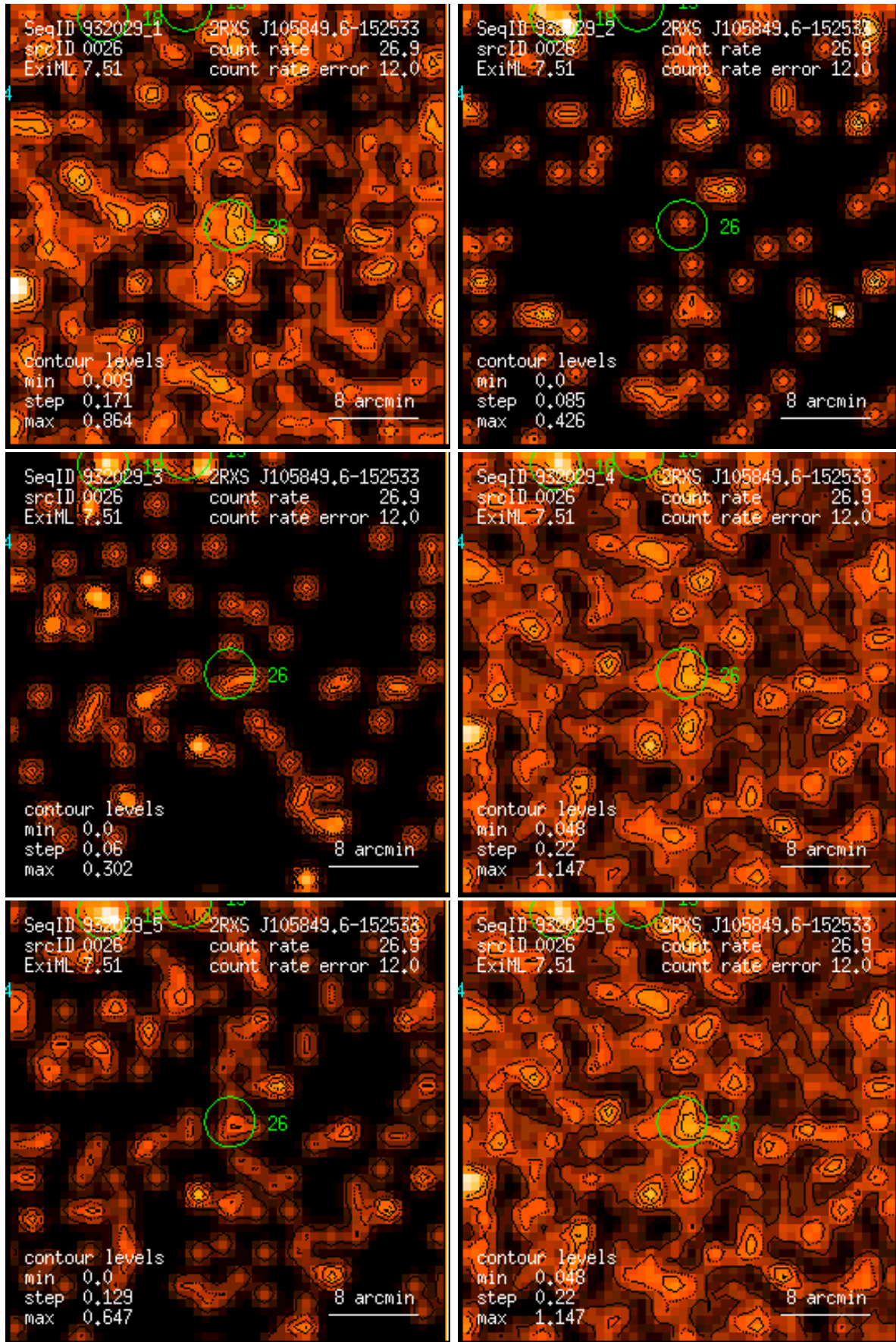
Figure 26: RASS 932029: detection 0026: band rate images, Gaussian filter: (1) PSPC channels 11 – 41, (2) 52 – 90, (3) 91 – 201, (4) 11 – 235, (5) 52 – 201, (6) 11 – 201. Broad band rates in counts/ks. Band rate contour levels in counts/ks/arcmin 2 .
