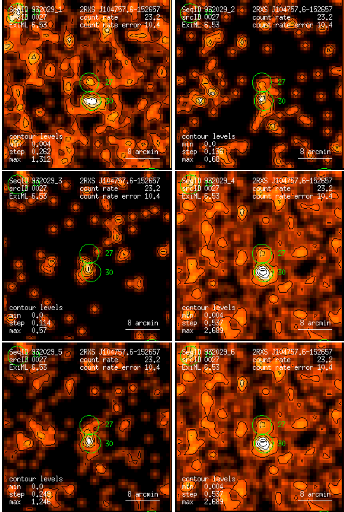
Figure 27: RASS 932029: detection 0027: band rate images, Gaussian filter: (1) PSPC channels 11 – 41, (2) 52 – 90, (3) 91 – 201, (4) 11 – 235, (5) 52 – 201, (6) 11 – 201. Broad band rates in counts/ks. Band rate contour levels in counts/ks/arcmin 2 .
