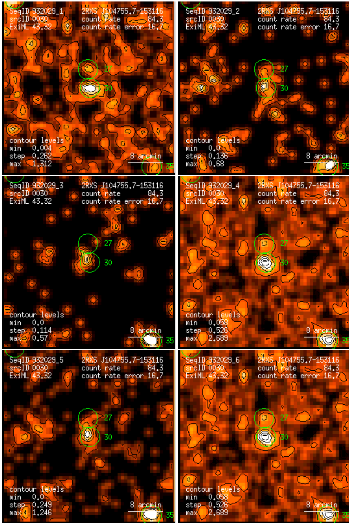
Figure 30: RASS 932029: detection 0030: band rate images, Gaussian filter: (1) PSPC channels 11 – 41, (2) 52 – 90, (3) 91 – 201, (4) 11 – 235, (5) 52 – 201, (6) 11 – 201. Broad band rates in counts/ks. Band rate contour levels in counts/ks/arcmin 2 .
