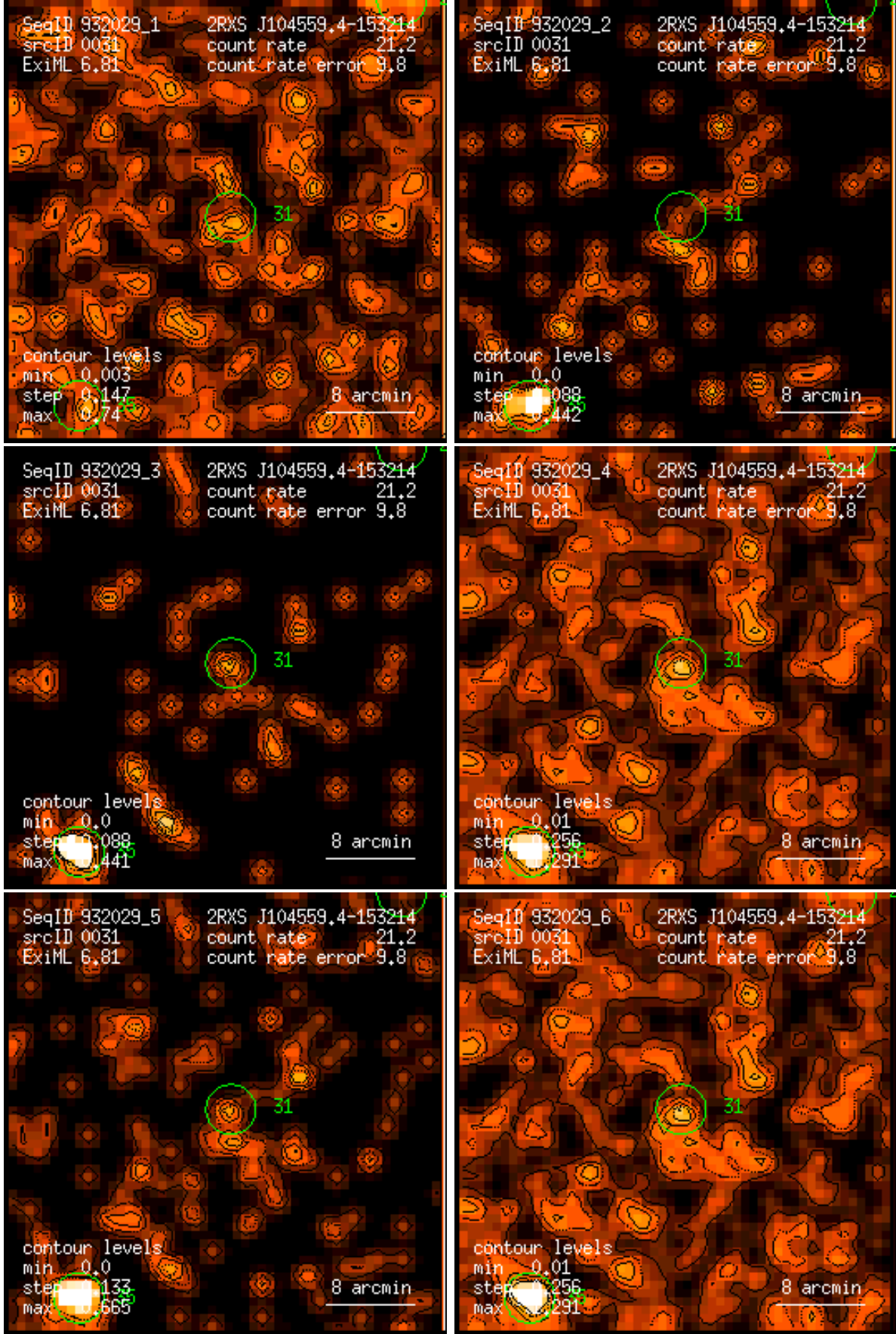
Figure 31: RASS 932029: detection 0031: band rate images, Gaussian filter: (1) PSPC channels 11 – 41, (2) 52 – 90, (3) 91 – 201, (4) 11 – 235, (5) 52 – 201, (6) 11 – 201. Broad band rates in counts/ks. Band rate contour levels in counts/ks/arcmin 2 .
