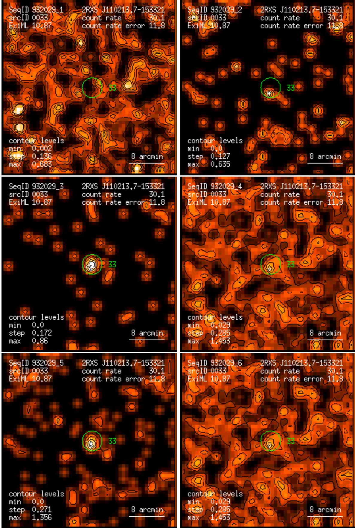
Figure 33: RASS 932029: detection 0033: band rate images, Gaussian filter: (1) PSPC channels 11 – 41, (2) 52 – 90, (3) 91 – 201, (4) 11 – 235, (5) 52 – 201, (6) 11 – 201. Broad band rates in counts/ks. Band rate contour levels in counts/ks/arcmin 2 .
