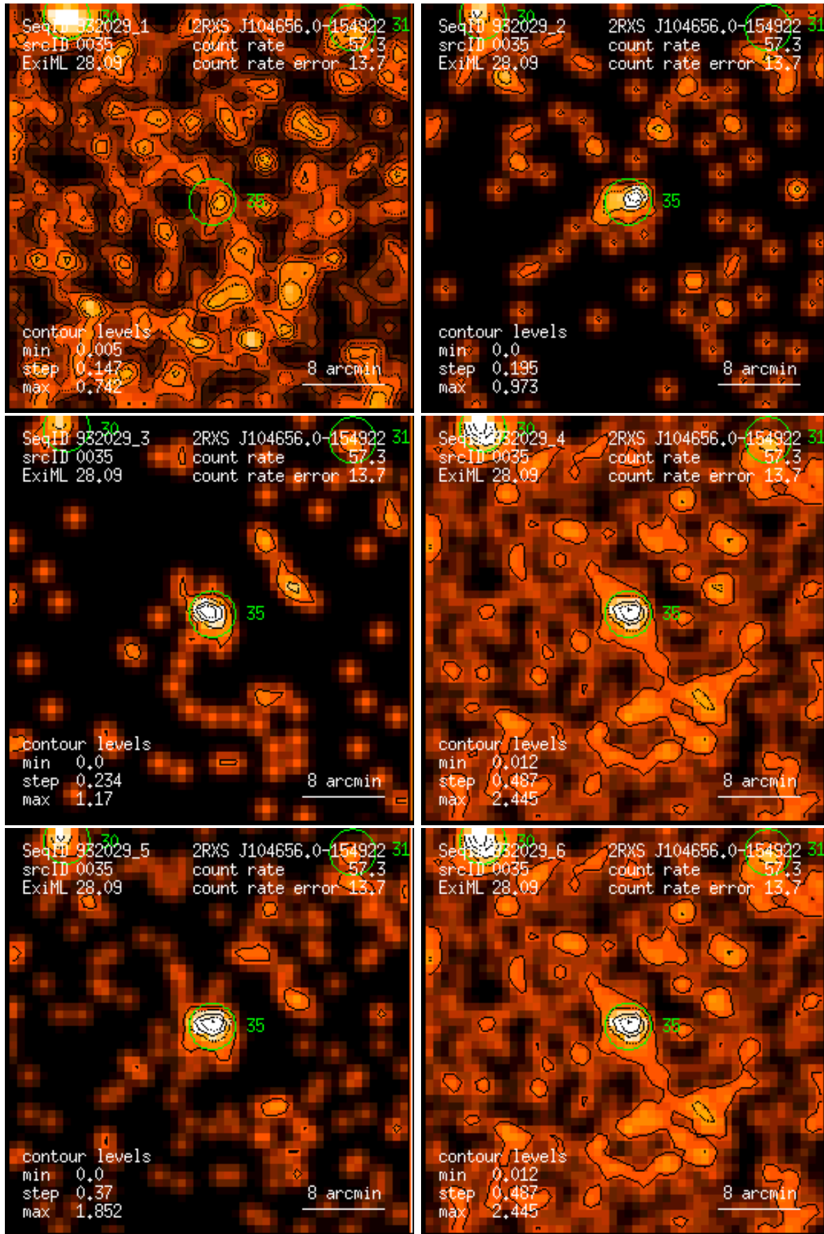
Figure 35: RASS 932029: detection 0035: band rate images, Gaussian filter: (1) PSPC channels 11 – 41, (2) 52 – 90, (3) 91 – 201, (4) 11 – 235, (5) 52 – 201, (6) 11 – 201. Broad band rates in counts/ks. Band rate contour levels in counts/ks/arcmin 2 .
