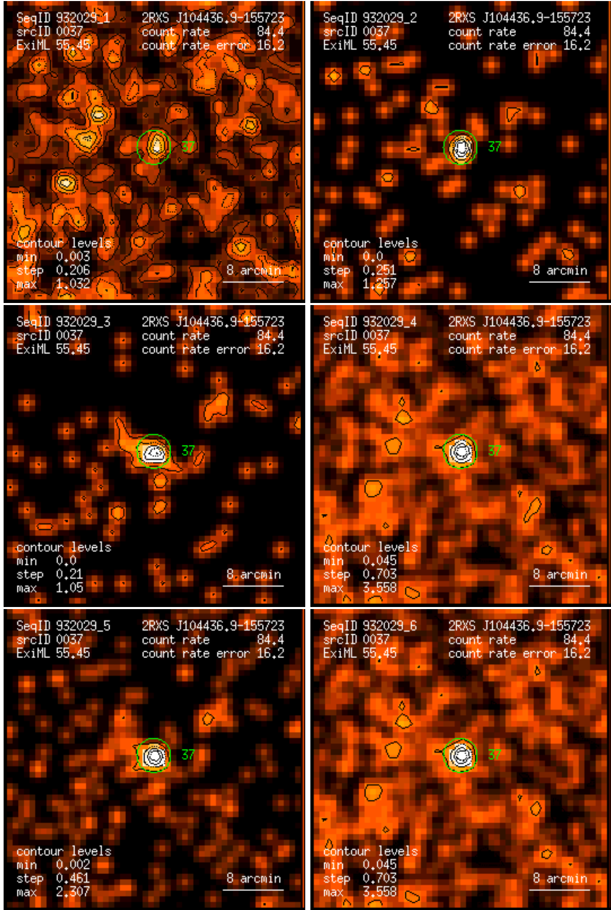
Figure 37: RASS 932029: detection 0037: band rate images, Gaussian filter: (1) PSPC channels 11 – 41, (2) 52 – 90, (3) 91 – 201, (4) 11 – 235, (5) 52 – 201, (6) 11 – 201. Broad band rates in counts/ks. Band rate contour levels in counts/ks/arcmin 2 .
