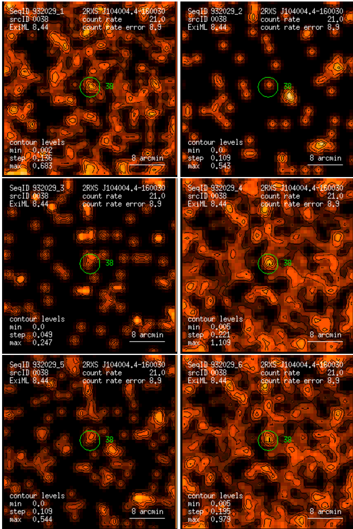
Figure 38: RASS 932029: detection 0038: band rate images, Gaussian filter: (1) PSPC channels 11 – 41, (2) 52 – 90, (3) 91 – 201, (4) 11 – 235, (5) 52 – 201, (6) 11 – 201. Broad band rates in counts/ks. Band rate contour levels in counts/ks/arcmin 2 .
