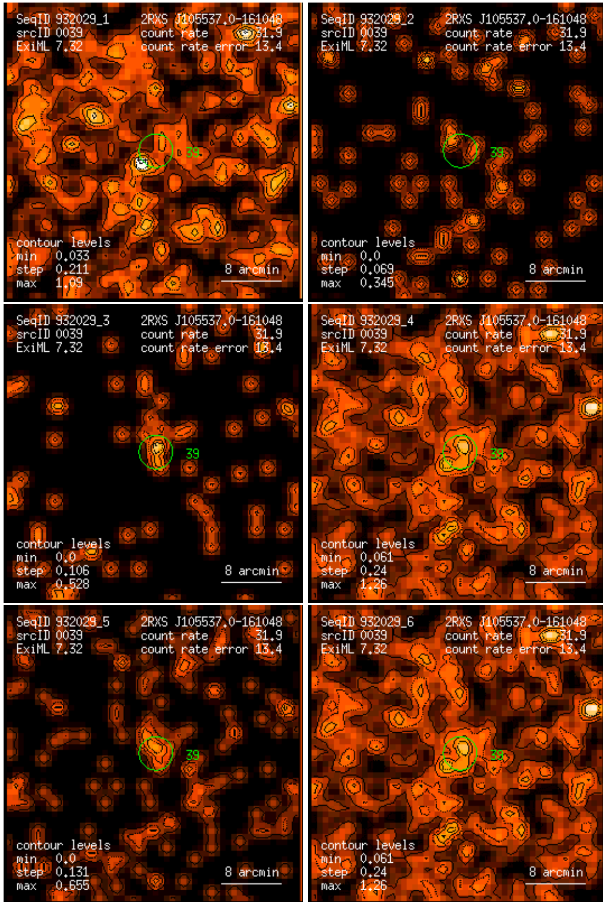
Figure 39: RASS 932029: detection 0039: band rate images, Gaussian filter: (1) PSPC channels 11 – 41, (2) 52 – 90, (3) 91 – 201, (4) 11 – 235, (5) 52 – 201, (6) 11 – 201. Broad band rates in counts/ks. Band rate contour levels in counts/ks/arcmin 2 .
