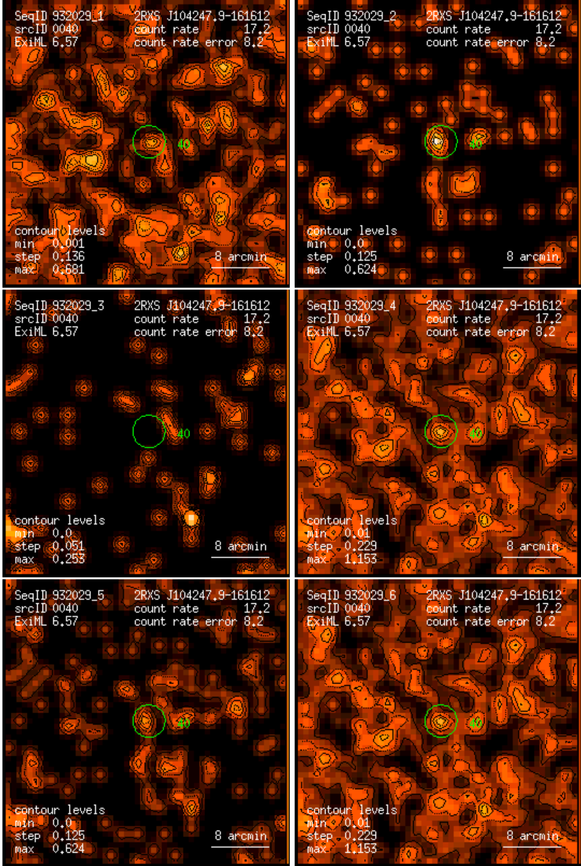
Figure 40: RASS 932029: detection 0040: band rate images, Gaussian filter: (1) PSPC channels 11 – 41, (2) 52 – 90, (3) 91 – 201, (4) 11 – 235, (5) 52 – 201, (6) 11 – 201. Broad band rates in counts/ks. Band rate contour levels in counts/ks/arcmin 2 .
