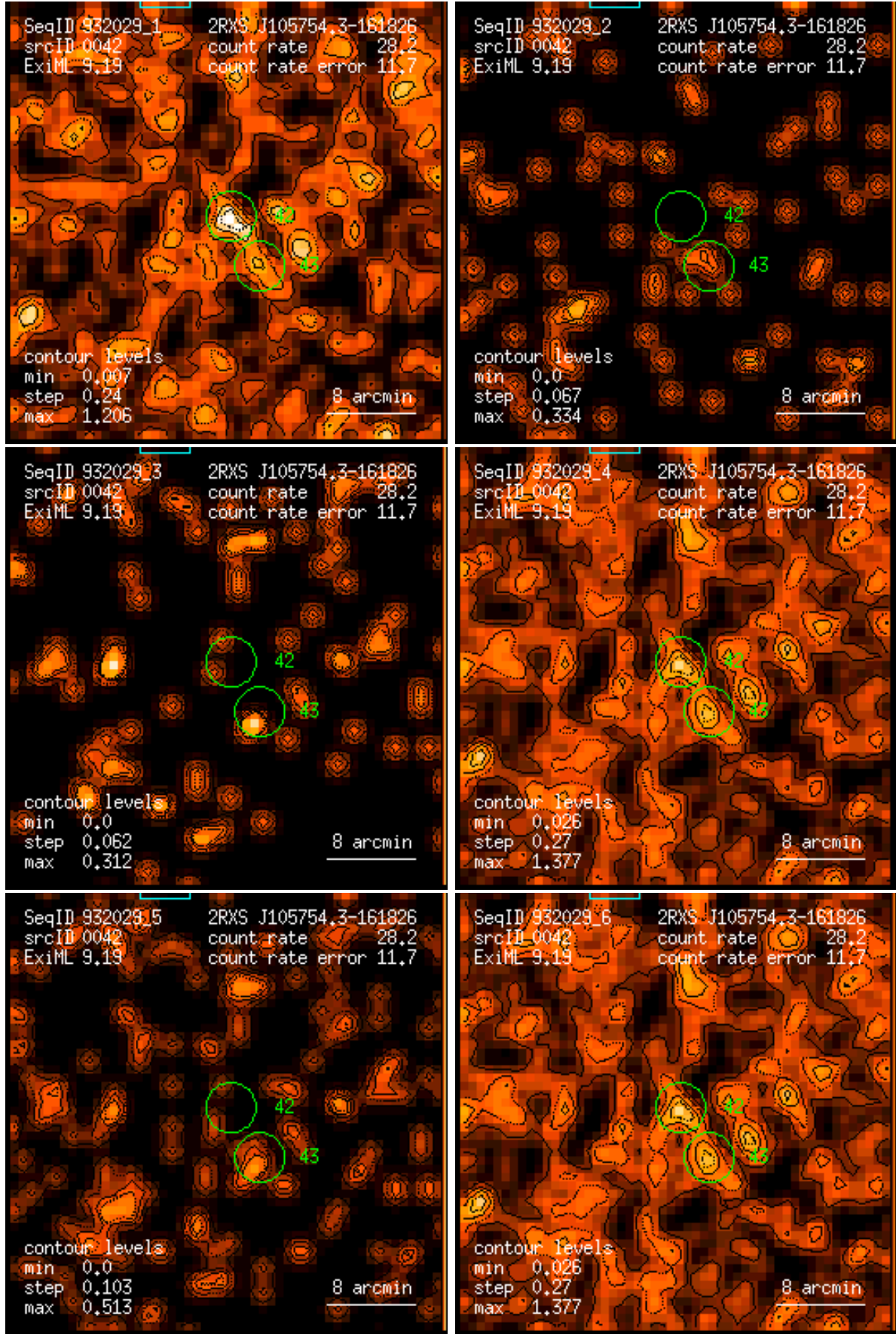
Figure 42: RASS 932029: detection 0042: band rate images, Gaussian filter: (1) PSPC channels 11 – 41, (2) 52 – 90, (3) 91 – 201, (4) 11 – 235, (5) 52 – 201, (6) 11 – 201. Broad band rates in counts/ks. Band rate contour levels in counts/ks/arcmin 2 .
