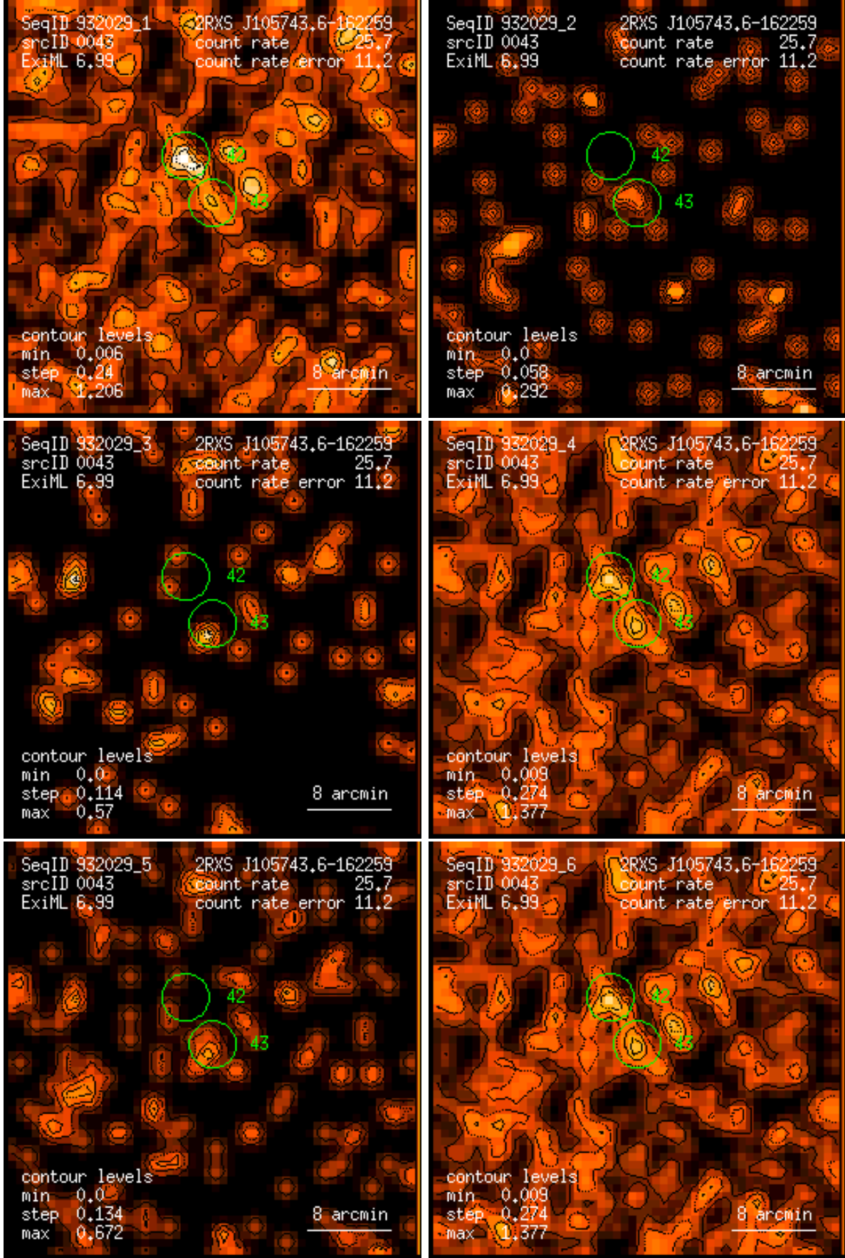
Figure 43: RASS 932029: detection 0043: band rate images, Gaussian filter: (1) PSPC channels 11 – 41, (2) 52 – 90, (3) 91 – 201, (4) 11 – 235, (5) 52 – 201, (6) 11 – 201. Broad band rates in counts/ks. Band rate contour levels in counts/ks/arcmin 2 .
