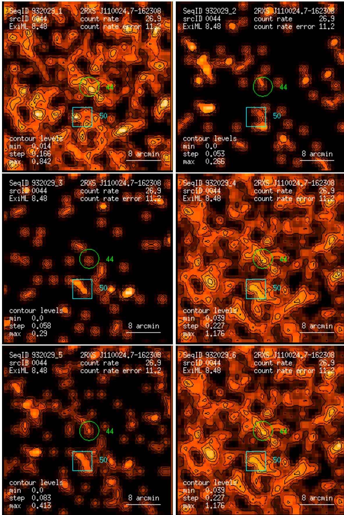
Figure 44: RASS 932029: detection 0044: band rate images, Gaussian filter: (1) PSPC channels 11 – 41, (2) 52 – 90, (3) 91 – 201, (4) 11 – 235, (5) 52 – 201, (6) 11 – 201. Broad band rates in counts/ks. Band rate contour levels in counts/ks/arcmin 2 .
