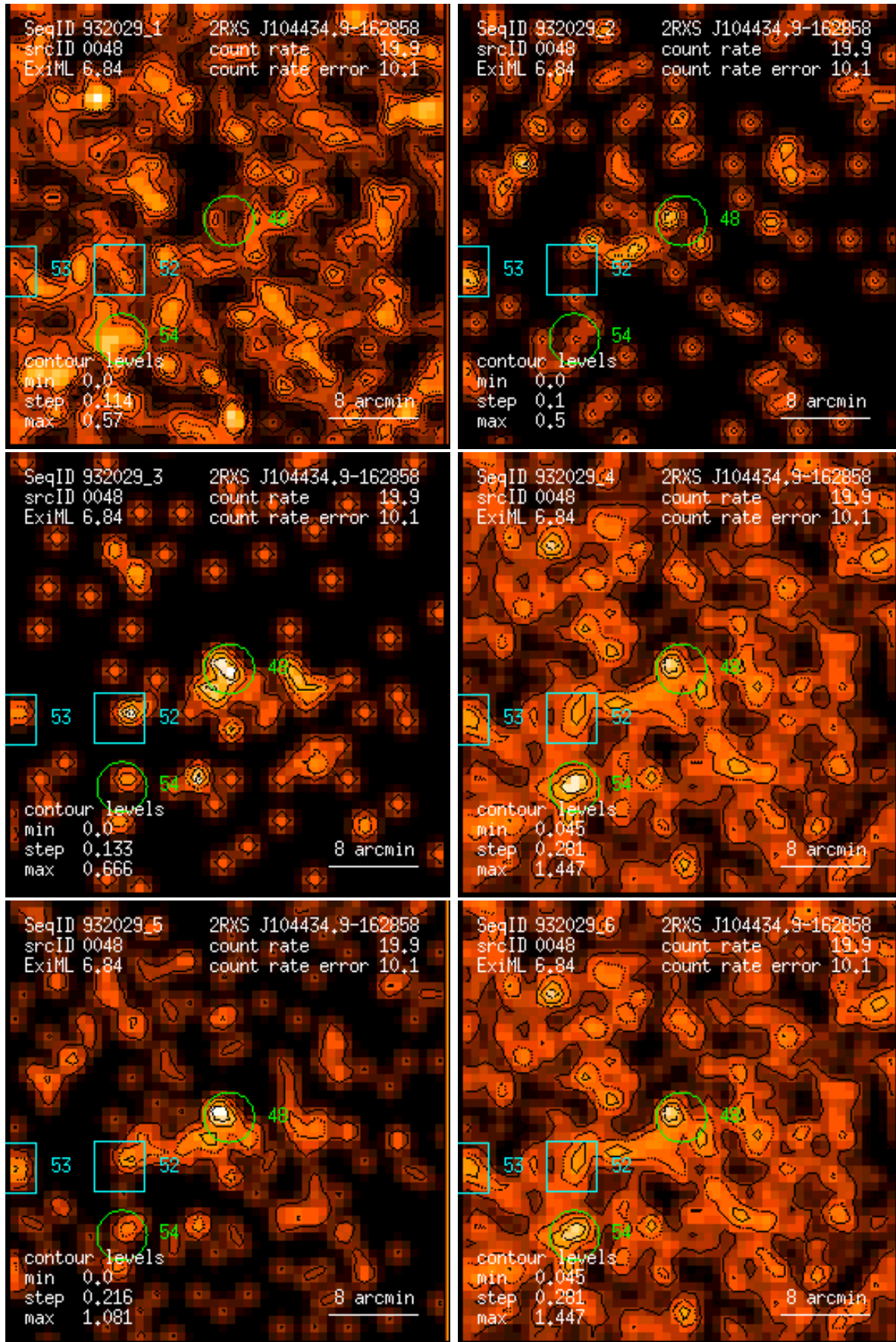
Figure 48: RASS 932029: detection 0048: band rate images, Gaussian filter: (1) PSPC channels 11 – 41, (2) 52 – 90, (3) 91 – 201, (4) 11 – 235, (5) 52 – 201, (6) 11 – 201. Broad band rates in counts/ks. Band rate contour levels in counts/ks/arcmin 2 .
