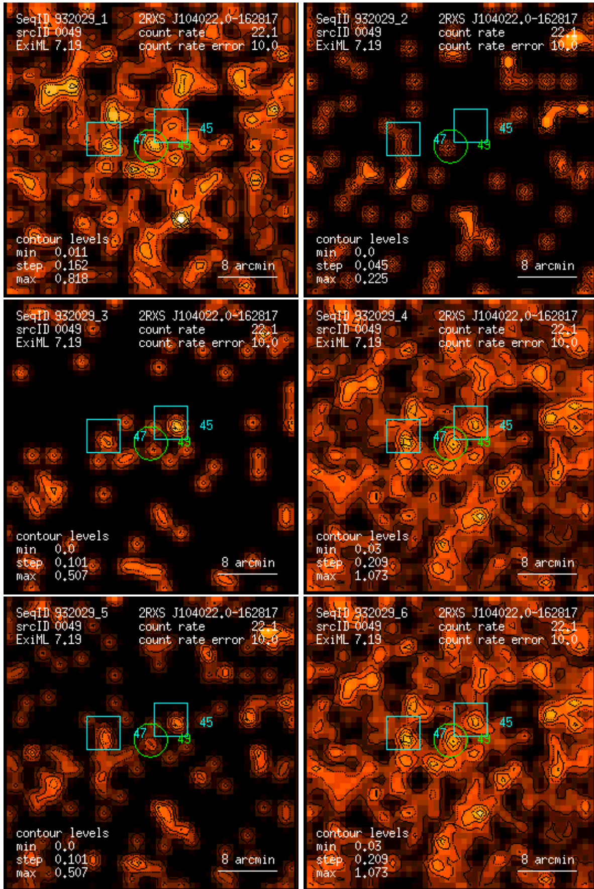
Figure 49: RASS 932029: detection 0049: band rate images, Gaussian filter: (1) PSPC channels 11 – 41, (2) 52 – 90, (3) 91 – 201, (4) 11 – 235, (5) 52 – 201, (6) 11 – 201. Broad band rates in counts/ks. Band rate contour levels in counts/ks/arcmin 2 .
