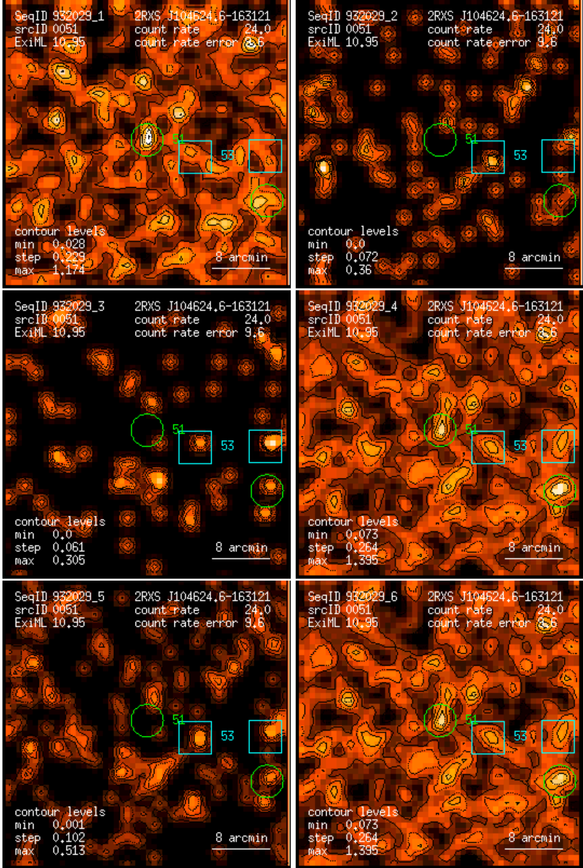
Figure 51: RASS 932029: detection 0051: band rate images, Gaussian filter: (1) PSPC channels 11 – 41, (2) 52 – 90, (3) 91 – 201, (4) 11 – 235, (5) 52 – 201, (6) 11 – 201. Broad band rates in counts/ks. Band rate contour levels in counts/ks/arcmin 2 .
