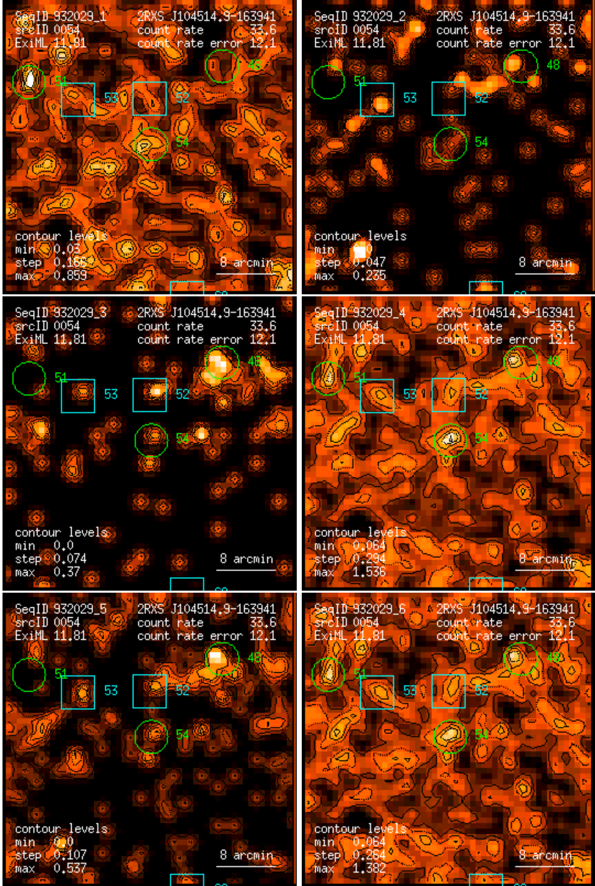
Figure 54: RASS 932029: detection 0054: band rate images, Gaussian filter: (1) PSPC channels 11 – 41, (2) 52 – 90, (3) 91 – 201, (4) 11 – 235, (5) 52 – 201, (6) 11 – 201. Broad band rates in counts/ks. Band rate contour levels in counts/ks/arcmin 2 .
