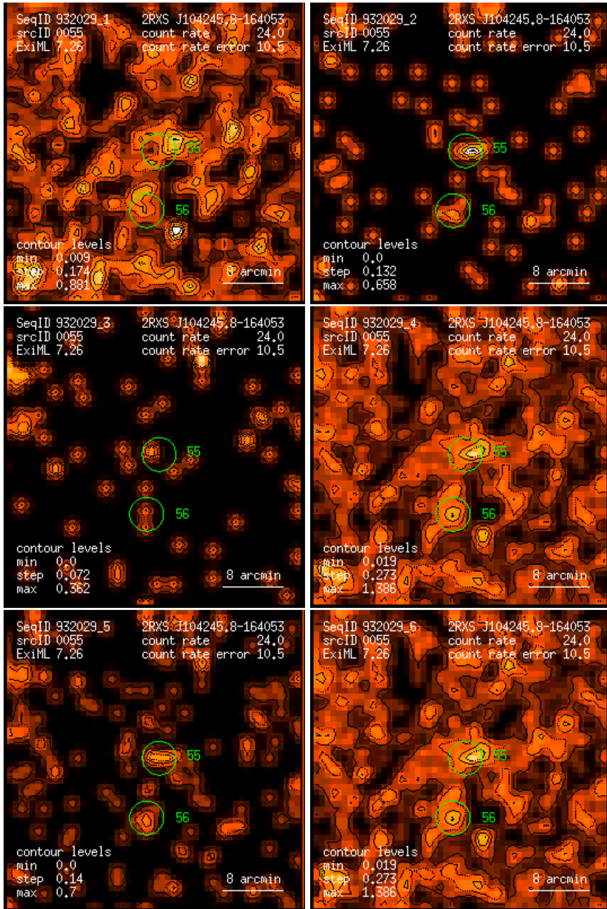
Figure 55: RASS 932029: detection 0055: band rate images, Gaussian filter: (1) PSPC channels 11 – 41, (2) 52 – 90, (3) 91 – 201, (4) 11 – 235, (5) 52 – 201, (6) 11 – 201. Broad band rates in counts/ks. Band rate contour levels in counts/ks/arcmin 2 .
