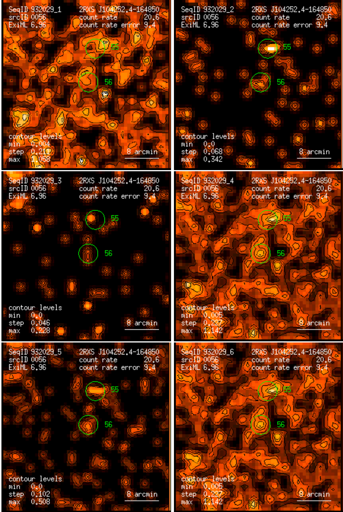
Figure 56: RASS 932029: detection 0056: band rate images, Gaussian filter: (1) PSPC channels 11 – 41, (2) 52 – 90, (3) 91 – 201, (4) 11 – 235, (5) 52 – 201, (6) 11 – 201. Broad band rates in counts/ks. Band rate contour levels in counts/ks/arcmin 2 .
