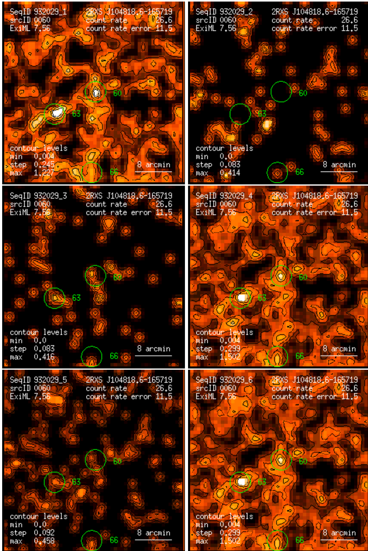
Figure 60: RASS 932029: detection 0060: band rate images, Gaussian filter: (1) PSPC channels 11 – 41, (2) 52 – 90, (3) 91 – 201, (4) 11 – 235, (5) 52 – 201, (6) 11 – 201. Broad band rates in counts/ks. Band rate contour levels in counts/ks/arcmin 2 .
