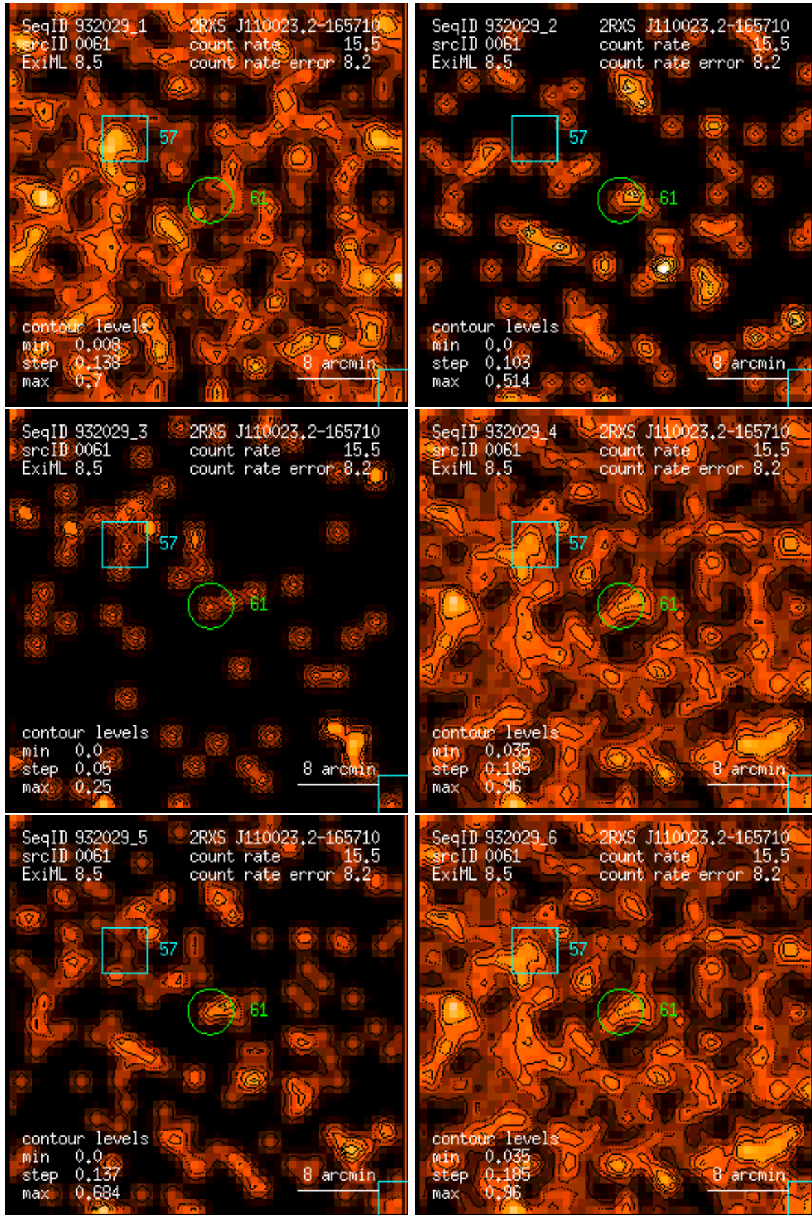
Figure 61: RASS 932029: detection 0061: band rate images, Gaussian filter: (1) PSPC channels 11 – 41, (2) 52 – 90, (3) 91 – 201, (4) 11 – 235, (5) 52 – 201, (6) 11 – 201. Broad band rates in counts/ks. Band rate contour levels in counts/ks/arcmin 2 .
