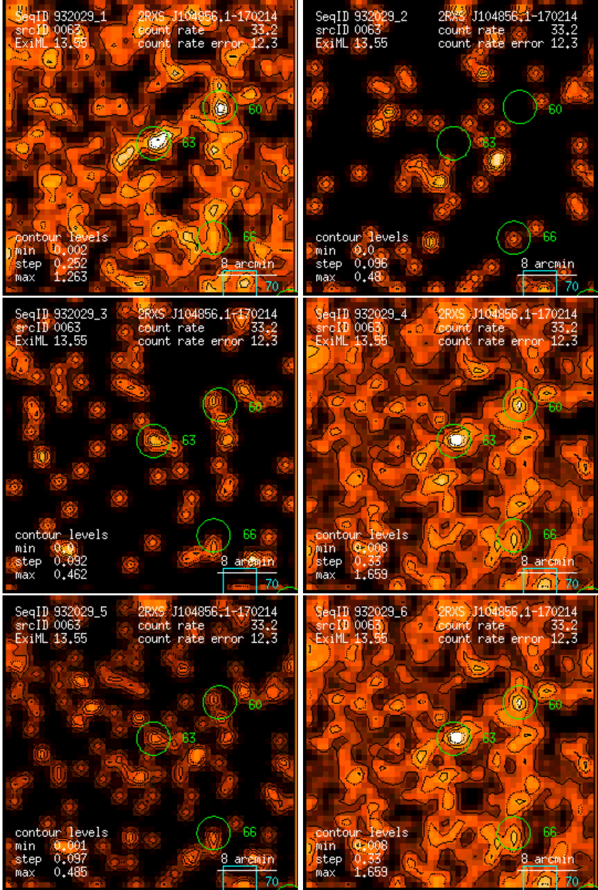
Figure 63: RASS 932029: detection 0063: band rate images, Gaussian filter: (1) PSPC channels 11 – 41, (2) 52 – 90, (3) 91 – 201, (4) 11 – 235, (5) 52 – 201, (6) 11 – 201. Broad band rates in counts/ks. Band rate contour levels in counts/ks/arcmin 2 .
